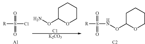
Scheme C. General Synthesis of Intermediate N-(tetrahydro-pyran-2-yloxy)sulfonamides.
