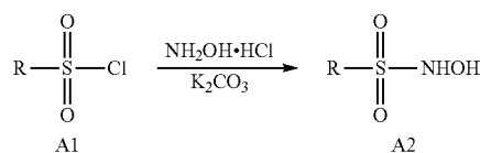
Scheme A. General Synthesis of N-Hydroxysulfonamides.
