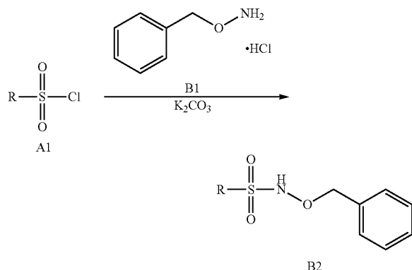
Scheme B. General Synthesis of Intermediate N-Benzoyloxysulfonamides.
