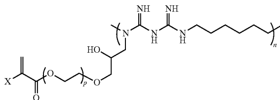
Structure 2
