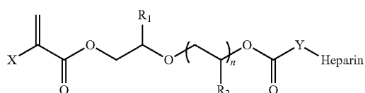
Structure 15
