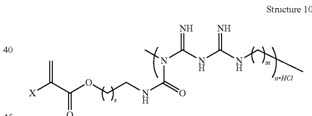
Structure 10
