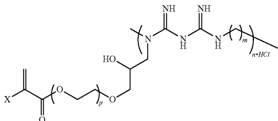
Structure 6
