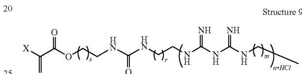
Structure 9
