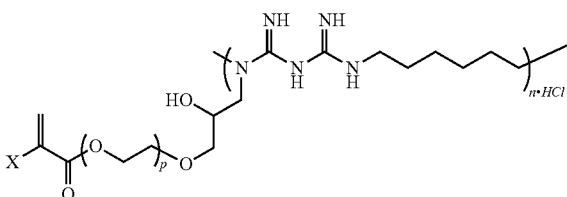
Structure 3
