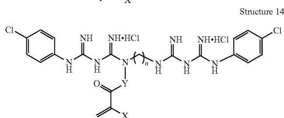
Structure 14
