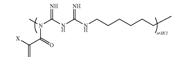
Structure 4
