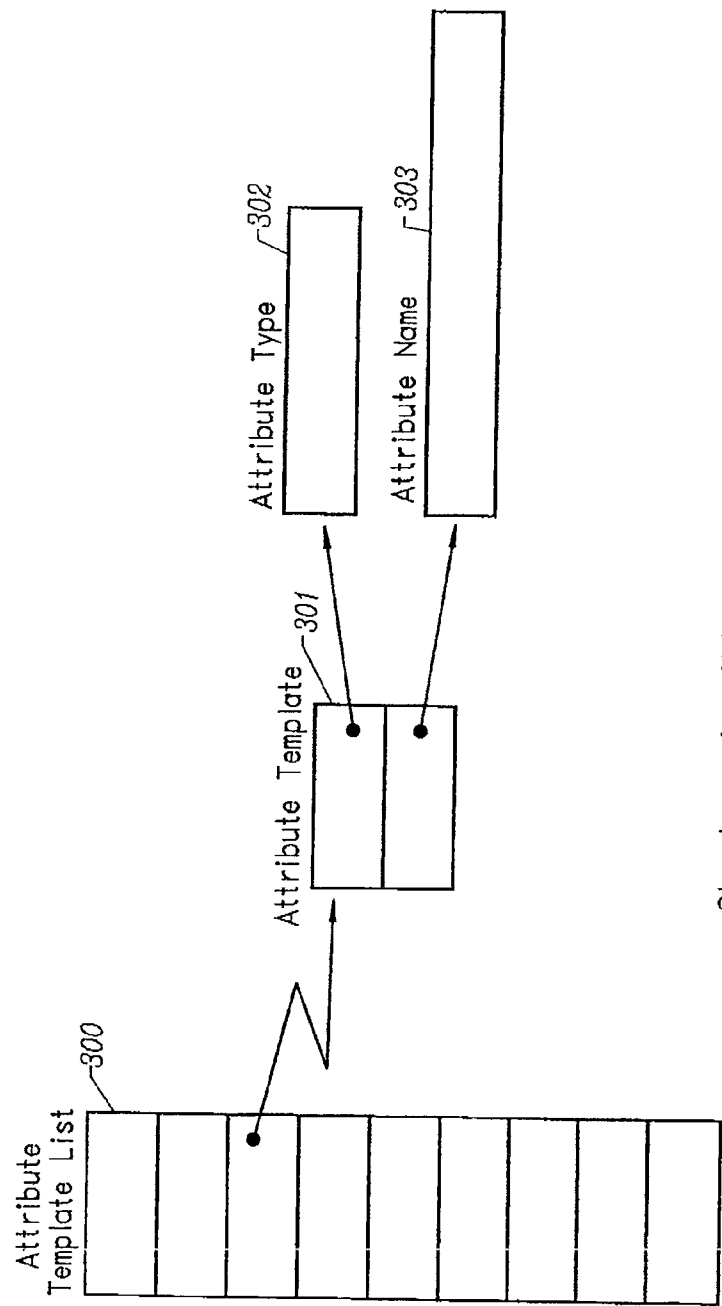
Structure of a Object Schema FIG. 3
