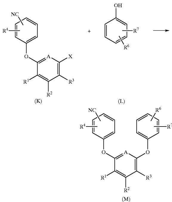
REACTION SCHEME 4
