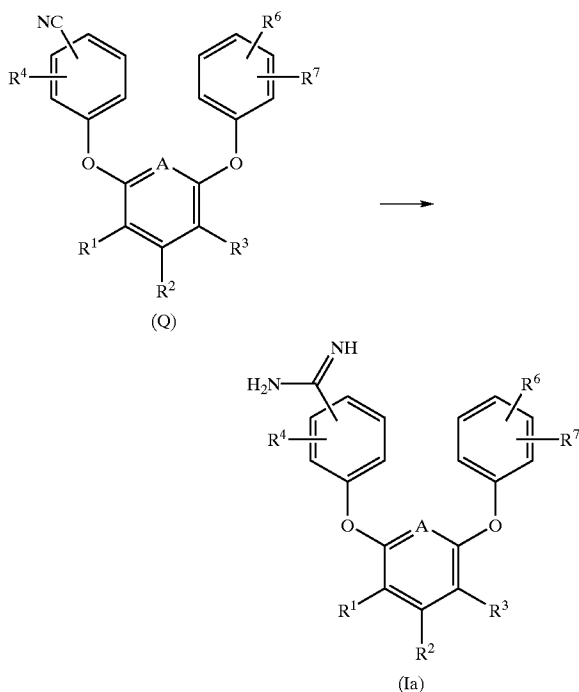
REACTION SCHEME 6
