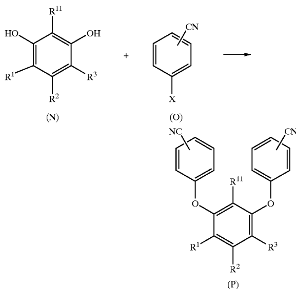
REACTION SCHEME 5
