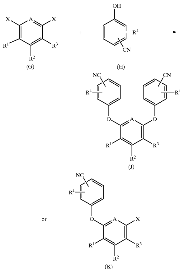
REACTION SCHEME 3
