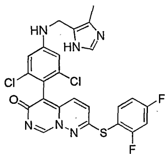
Compound 11,
