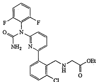
Compound 18.
