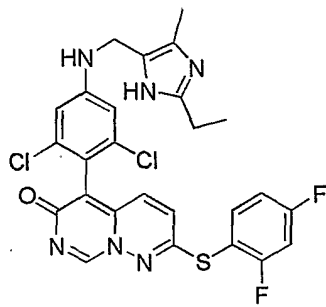
Compound 12,
