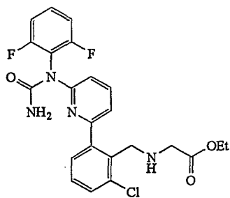
Compound 18
