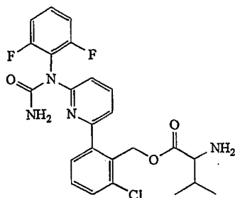
Compound 16.
