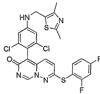
Compound 13, and
