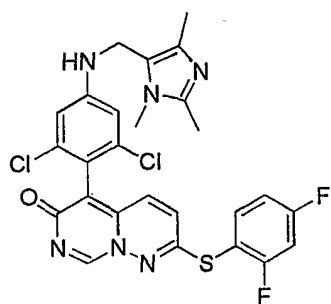
5 Compound 14.
