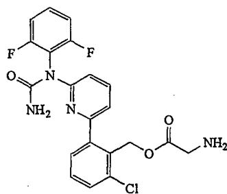
Compound 15
