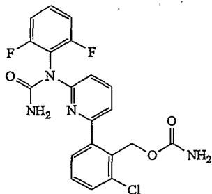
Compound 17.
