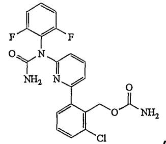
Compound 17
