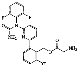
Compound 15.
