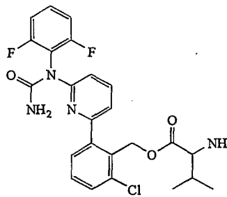
Compound 16
