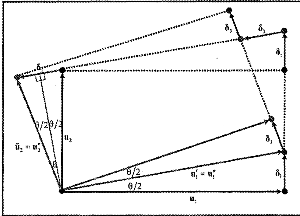
Figure 3: Geometry used to determine skews that result in a \theta rotation
