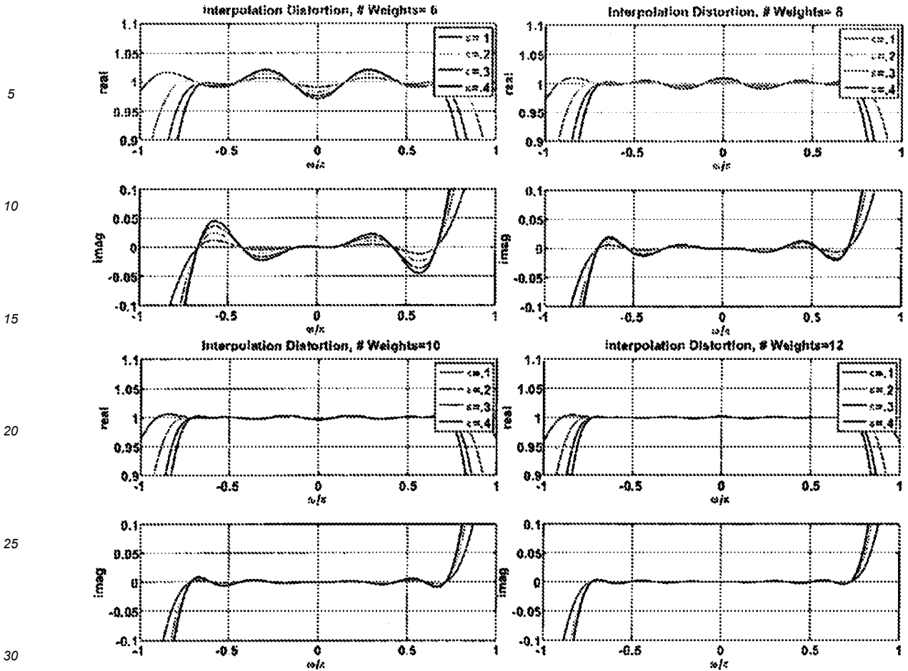
Figure 7: Distortion curves of interpolations at fractional offsets of 0.1, 0.2, 0.3 and 0.4 using coefficients giving minimum least-square error in the frequency band [-0.75\pi, +0.75\pi] . The four panels show the distortion for interpolation filters with 6 (upper left), 8 (upper right), 10 (lower left) and 12 (lower right) coefficients.
