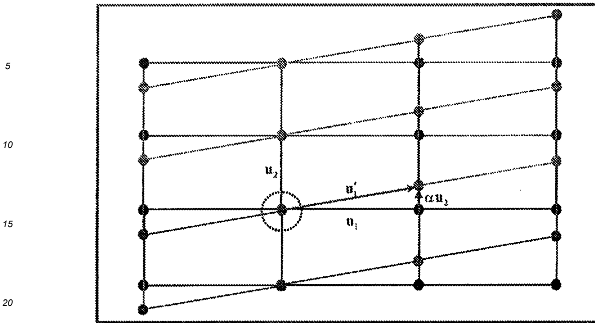
Figure 1: Coordinate transformation produced by skewing the horizontal generating vector
