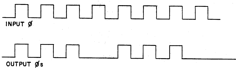
INPUT / OUTPUT OF A TWO STAGE BRM
