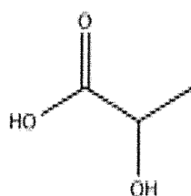
Lactic Acid
