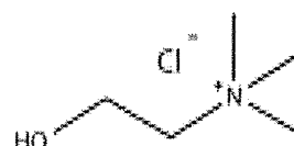
Choline Chloride
