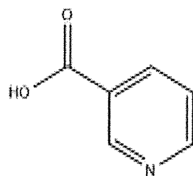
Nicotinic Acid
