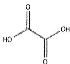
Oxalic Acid
