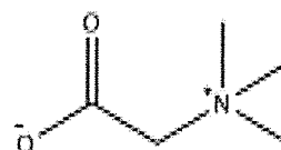
Betaine
