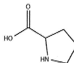
Proline
