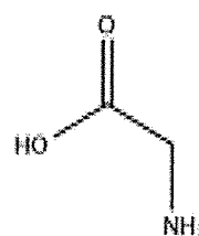
Glycine
