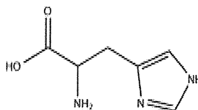
Histidine
