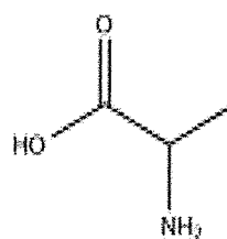
Alanine
