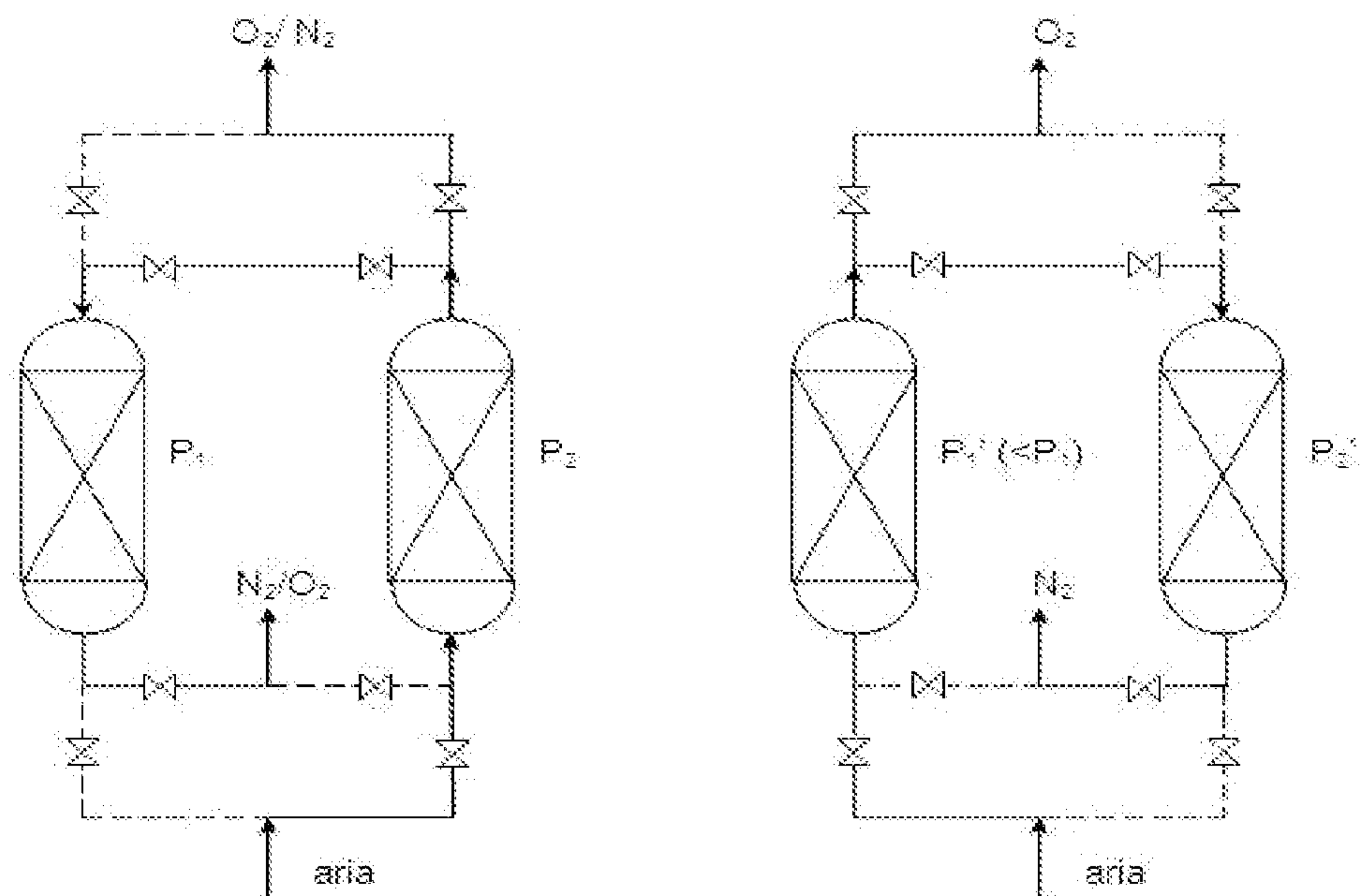
FIG 1 Pressure Swing Adsorption
