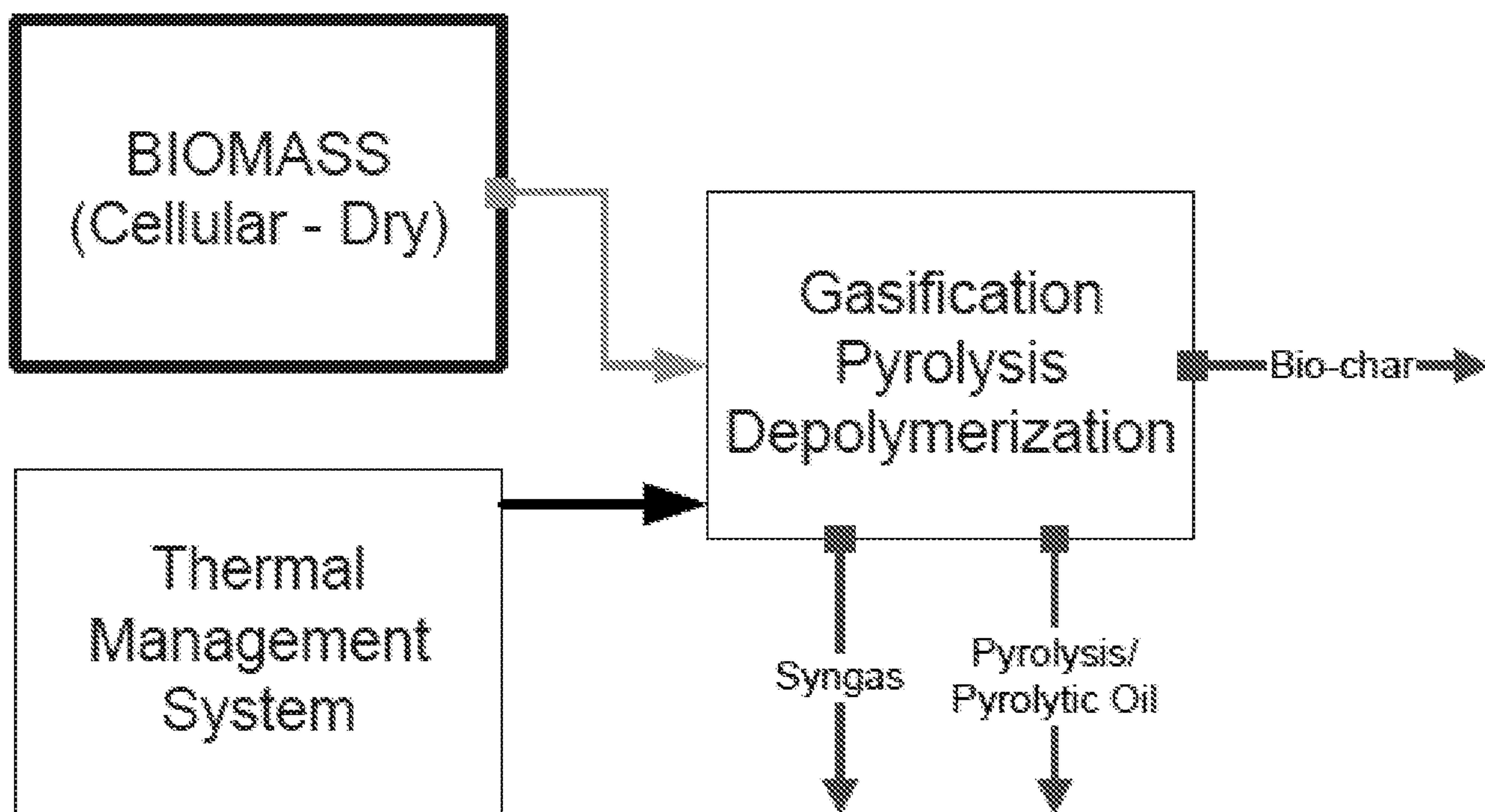
FIG 14 Thermochemical Processing
