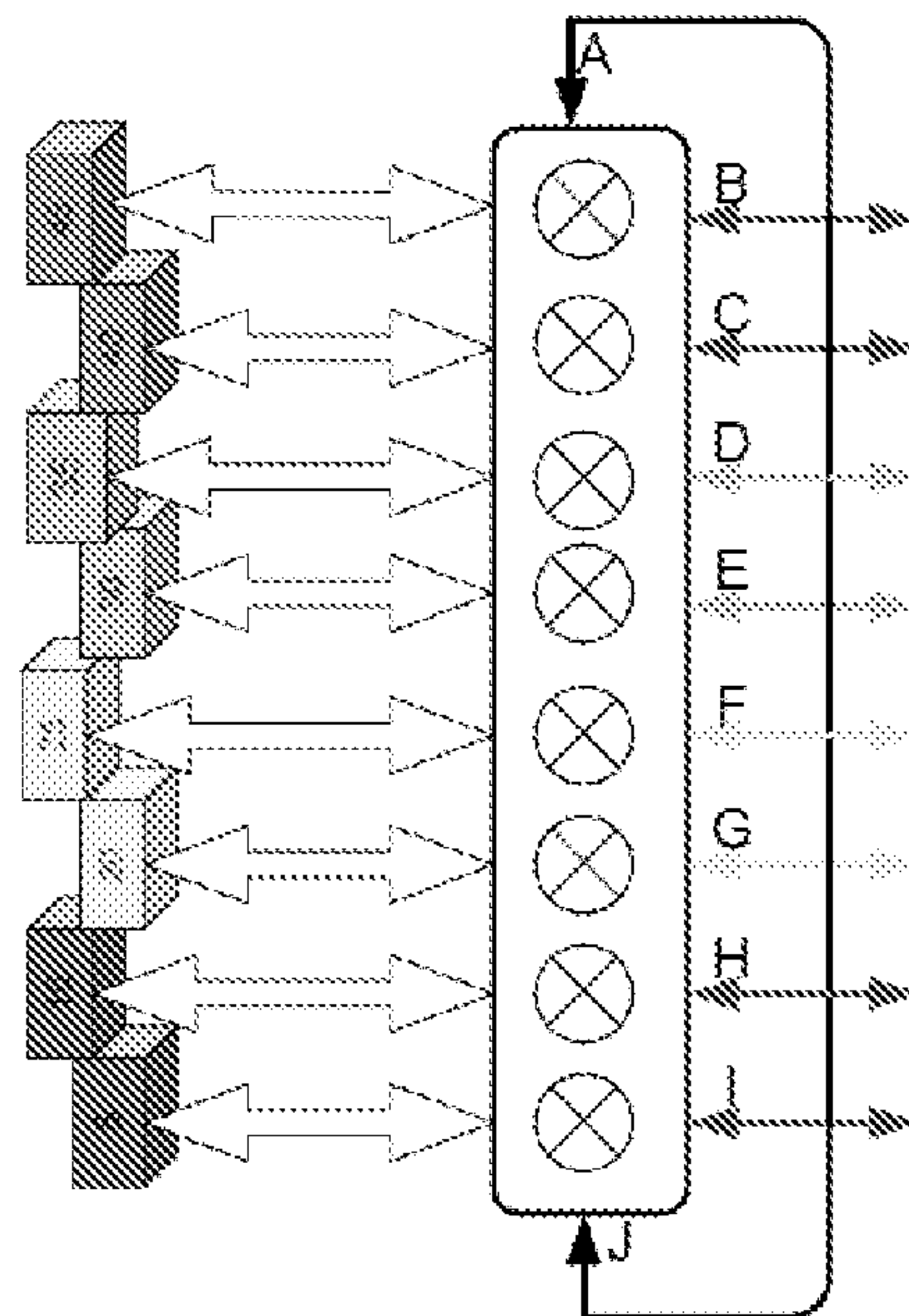
FIG 10B Temperature Gradient Heat Exchanger
