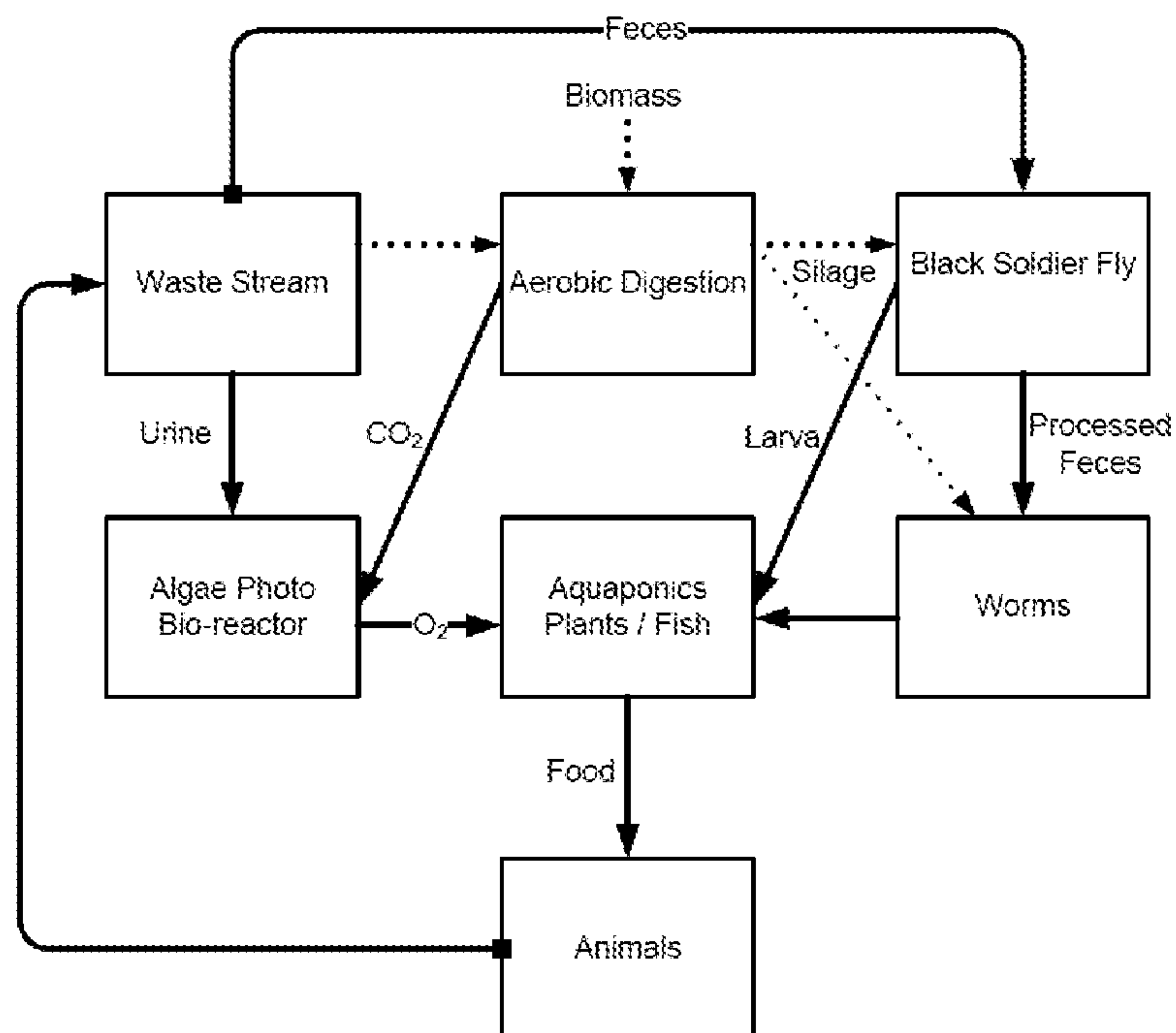
FIG 12 Waste Streams
