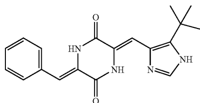
tBu-dehydrophenylahistin
