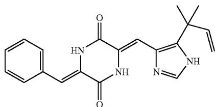
Dehydrophenylahistin
