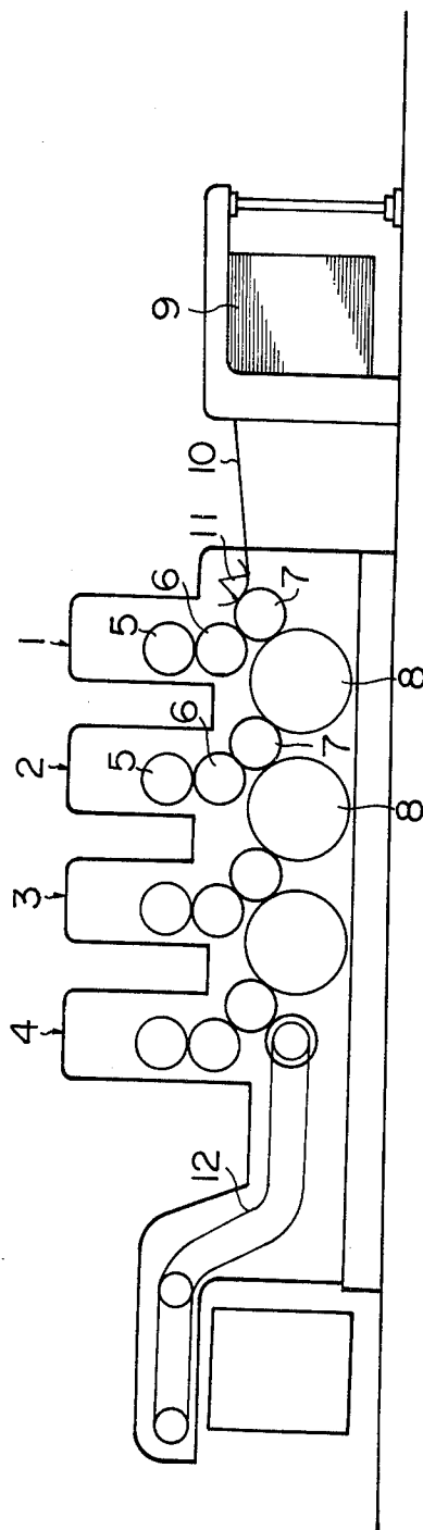
FIG. 2 PRIOR ART
