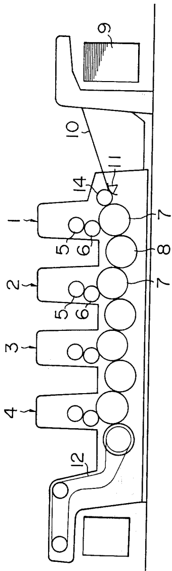
FIG. 3 PRIOR ART
