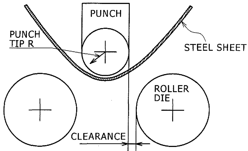
SCHEMATIC VIEW OF THREE-POINT U-BENDING TEST
