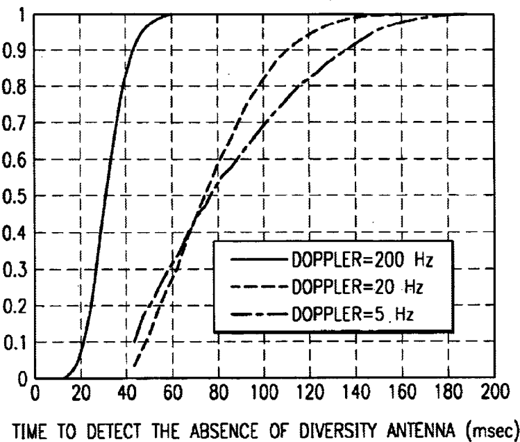
CUMULATIVE PROBABILITY OF TIME TO DETECT ABSENCE OF DIVERSITY ANTENNA
