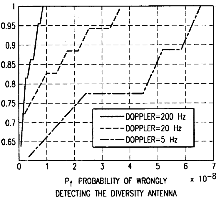
CUMULATIVE PROBABILITY OF P_f
