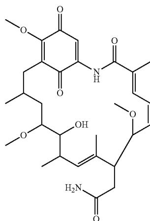
Geldanamycin CAS number: 30562-34-6 Molecular Weight: 560.6
