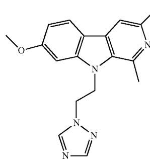
9-(2-(1H-1,2,4-triazol-1-yl)ethyl)-3-fluoro-7-methoxy-1-methyl-9H-pyrido[3,4-b]indole;
