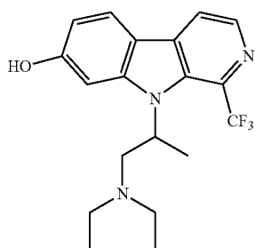
9-(1-(diethylamino)propan-2-yl)-1-(trifluoromethyl)-9H-pyrido[3,4-b]indol-7-ol;
