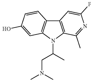
9-(1-(dimethylamino)propan-2-yl)-3-fluoro-1-methyl-9H-pyrido[3,4-b]indol-7-ol;
