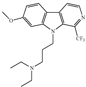
N,N-diethyl-3-(7-methoxy-1-(trifluoromethyl)-9H-pyrido[3,4-b]indol-9-yl)propan-1-amine;
