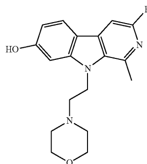
3-fluoro-1-methyl-9-(2-morpholinoethyl)-9H-pyrido[3,4-b]indol-7-ol;
