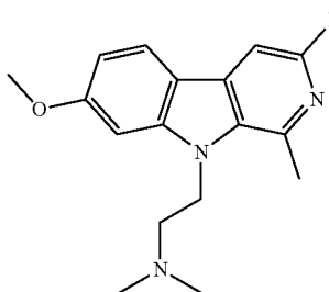
2-(3-fluoro-7-methoxy-1-methyl-9H-pyrido[3,4-b]indol-9-yl)-N,N-dimethylethanamine;
