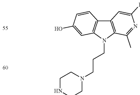
3-fluoro-1-methyl-9-(3-(piperazin-1-yl)propyl)-9H-pyrido[3,4-b]indol-7-ol;
