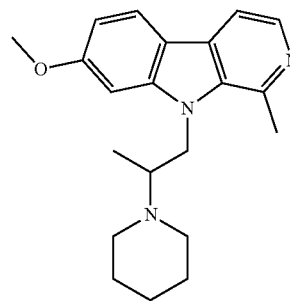
7-methoxy-1-methyl-9-(2-(piperidin-1-yl)propyl)-9H-pyrido[3,4-b]indole;
