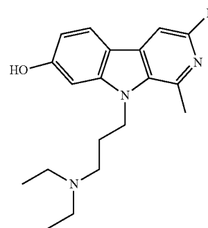
9-(3-(diethylamino)propyl)-3-fluoro-1-methyl-9H-pyrido[3,4-b]indol-7-ol;
