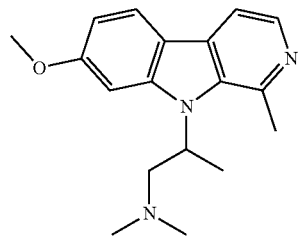
2-(7-methoxy-1-(trifluoromethyl)-9H-pyrido[3,4-b]indol-9-yl)-N,N-dimethylpropan-1-amine;
