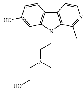
9-(2-((2-hydroxyethyl)(methyl)amino)ethyl)-1-methyl-9H-pyrido[3,4-b]indol-7-ol;
