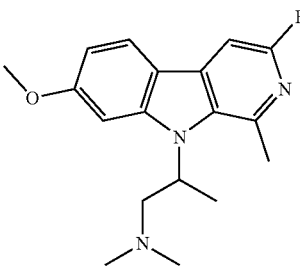
2-(7-methoxy-1-methyl-9H-pyrido[3,4-b]indol-9-yl)-N,N-dimethylpropan-1-amine;
