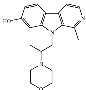
1-methyl-9-(2-morpholinopropyl)-9H-pyrido[3,4-b]indol-7-ol;
