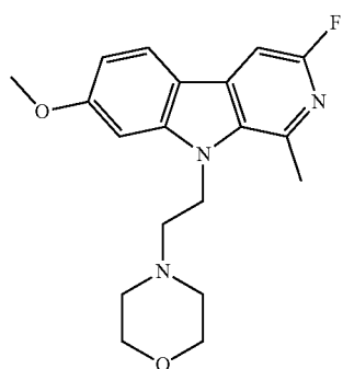
4-(2-(3-fluoro-7-methoxy-1-methyl-9H-pyrido[3,4-b]indol-9-yl)ethyl)morpholine;
