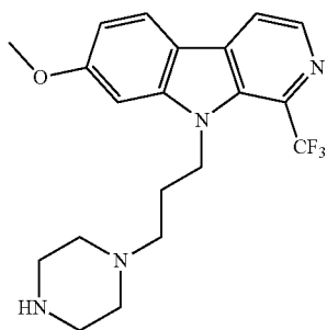
7-methoxy-9-(3-(piperazin-1-yl)propyl)-1-(trifluoromethyl)-9H-pyrido[3,4-b]indole;
