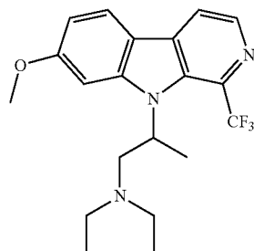
15 N,N-diethyl-2-(7-methoxy-1-(trifluoromethyl)-9H-pyrido[3,4-b]indol-9-yl)propan-1-amine;
