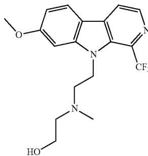
2-((2-(7-methoxy-1-(trifluoromethyl)-9H-pyrido[3,4-b]indol-9-yl)ethyl)(methyl)amino)ethanol;
