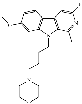
4-(4-(3-fluoro-7-methoxy-1-methyl-9H-pyrido[3,4-b]indol-9-yl)butyl)morpholine;
