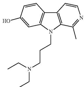
9-(3-(diethylamino)propyl)-1-methyl-9H-pyrido[3,4-b]indol-7-ol;
