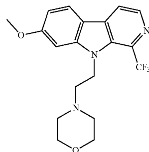
4-(2-(7-methoxy-1-(trifluoromethyl)-9H-pyrido[3,4-b]indol-9-yl)ethyl)morpholine;
