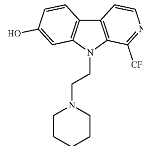
9-(2-(piperidin-1-yl)ethyl)-1-(trifluoromethyl)-9H-pyrido[3,4-b]indol-7-ol;
