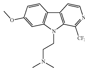
9-(2-(dimethylamino)ethyl)-3-fluoro-1-methyl-9H-pyrido[3,4-b]indol-7-ol;
