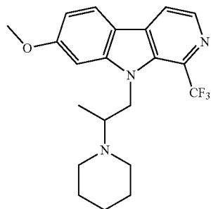
7-methoxy-9-(2-(piperidin-1-yl)propyl)-1-(trifluoromethyl)-9H-pyrido[3,4-b]indole;
