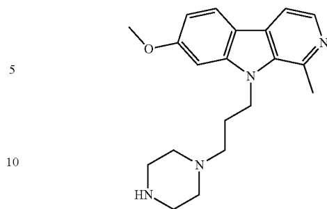
7-methoxy-1-methyl-9-(3-(piperazin-1-yl)propyl)-9H-pyrido[3,4-b]indole;
