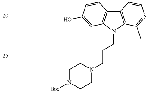
tert-butyl 4-(3-(7-hydroxy-1-methyl-9H-pyrido[3,4-b]indol-9-yl)propyl)piperazine-1-carboxylate;
