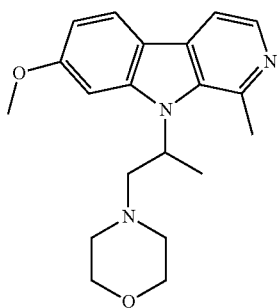
4-(2-(7-methoxy-1-methyl-9H-pyrido[3,4-b]indol-9-yl)propyl)morpholine;
