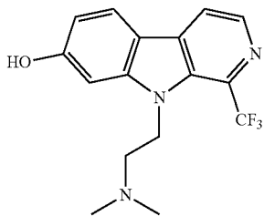
9-(2-(dimethylamino)ethyl)-1-(trifluoromethyl)-9H-pyrido[3,4-b]indol-7-ol;
