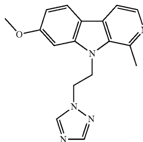
9-(2-(1H-1,2,4-triazol-1-yl)ethyl)-7-methoxy-1-methyl-9H-pyrido[3,4-b]indole;
