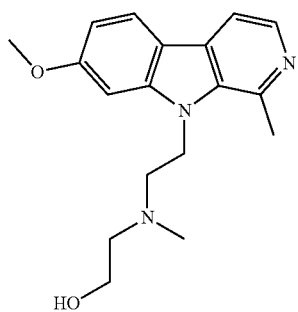
2-((2-(7-methoxy-1-methyl-9H-pyrido[3,4-b]indol-9-yl)ethyl)(methyl)amino)ethanol;
