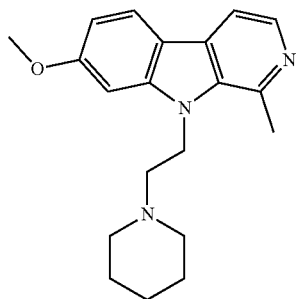
7-methoxy-1-methyl-9-(2-(piperidin-1-yl)ethyl)-9H-pyrido[3,4-b]indole;
