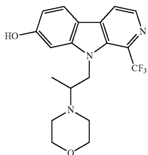
9-(2-morpholinopropyl)-1-(trifluoromethyl)-9H-pyrido[3,4-b]indol-7-ol;
