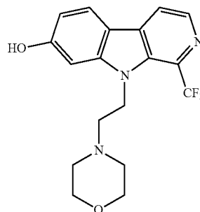
9-(2-morpholinoethyl)-1-(trifluoromethyl)-9H-pyrido[3,4-b]indol-7-ol;
