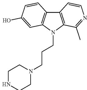
1-methyl-9-(3-(piperazin-1-yl)propyl)-9H-pyrido[3,4-b]indol-7-ol;
