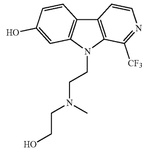
9-(2-((2-hydroxyethyl)(methyl)amino)ethyl)-1-(trifluoromethyl)-9H-pyrido[3,4-b]indol-7-ol;
