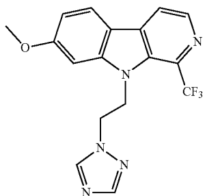
9-(2-(1H-1,2,4-triazol-1-yl)ethyl)-7-methoxy-1-(trifluoromethyl)-9H-pyrido[3,4-b]indole;
