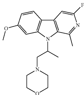
4-(2-(3-fluoro-7-methoxy-1-methyl-9H-pyrido[3,4-b]indol-9-yl)propyl)morpholine;
