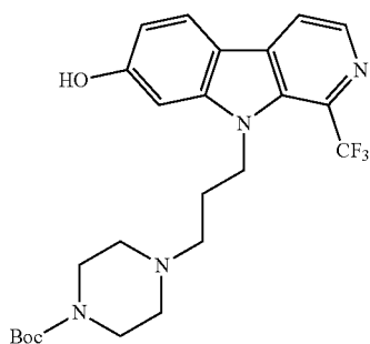
tert-butyl 4-(3-(7-hydroxy-1-(trifluoromethyl)-9H-pyrido[3,4-b]indol-9-yl)propyl)piperazine-1-carboxylate;
