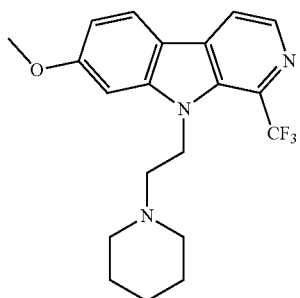
7-methoxy-9-(2-(piperidin-1-yl)ethyl)-1-(trifluoromethyl)-9H-pyrido[3,4-b]indole;
