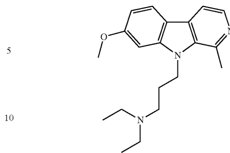
15 N,N-diethyl-3-(7-methoxy-1-methyl-9H-pyrido[3,4-b]indol-9-yl)propan-1-amine;
