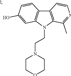
1-methyl-9-(2-morpholinoethyl)-9H-pyrido[3,4-b]indol-7-ol;
