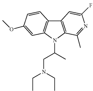
N,N-diethyl-2-(3-fluoro-7-methoxy-1-methyl-9H-pyrido[3,4-b]indol-9-yl)propan-1-amine;
