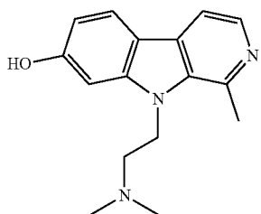
9-(2-(dimethylamino)ethyl)-1-methyl-9H-pyrido[3,4-b]indol-7-ol;
