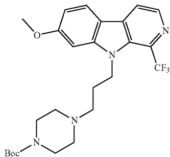
tert-butyl 4-(3-(7-methoxy-1-(trifluoromethyl)-9H-pyrido[3,4-b]indol-9-yl)propyl)piperazine-1-carboxylate;
