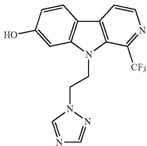
9-(2-(1H-1,2,4-triazol-1-yl)ethyl)-1-(trifluoromethyl)-9H-pyrido[3,4-b]indol-7-ol;
