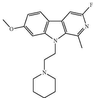
7-methoxy-1-methyl-9-(2-(piperidin-1-yl)ethyl)-9H-pyrido[3,4-b]indole;
