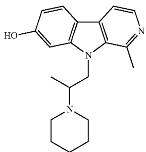
1-methyl-9-(2-(piperidin-1-yl)propyl)-9H-pyrido[3,4-b]indol-7-ol;
