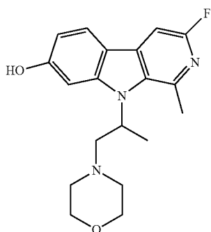
3-fluoro-1-methyl-9-(1-morpholinopropan-2-yl)-9H-pyrido[3,4-b]indol-7-ol;
