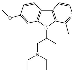
50 N,N-diethyl-2-(7-methoxy-1-methyl-9H-pyrido[3,4-b]indol-9-yl)propan-1-amine;
