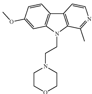
4-(2-(7-methoxy-1-methyl-9H-pyrido[3,4-b]indol-9-yl)ethyl)morpholine;
