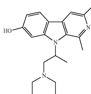
9-(1-(diethylamino)propan-2-yl)-3-fluoro-1-methyl-9H-pyrido[3,4-b]indol-7-ol;
