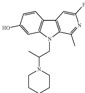
3-fluoro-1-methyl-9-(2-(piperidin-1-yl)propyl)-9H-pyrido[3,4-b]indol-7-ol;
