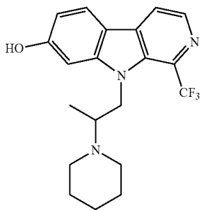
9-(2-(piperidin-1-yl)propyl)-1-(trifluoromethyl)-9H-pyrido[3,4-b]indol-7-ol;
