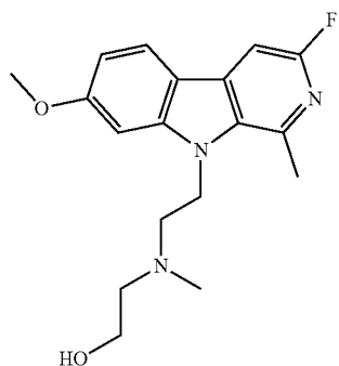
2-((2-(7-methoxy-1-methyl-9H-pyrido[3,4-b]indol-9-yl)ethyl)(methyl)amino)ethanol;
