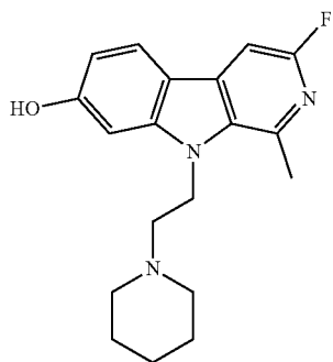
3-fluoro-1-methyl-9-(2-(piperidin-1-yl)ethyl)-9H-pyrido[3,4-b]indol-7-ol;
