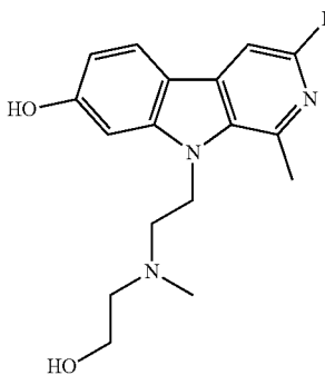
3-fluoro-9-(2-((2-hydroxyethyl)(methyl)amino)ethyl)-1-methyl-9H-pyrido[3,4-b]indol-7-ol;
