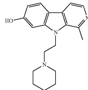
1-methyl-9-(2-(piperidin-1-yl)ethyl)-9H-pyrido[3,4-b]indol-7-ol;
