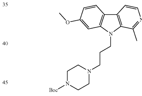
tert-butyl 4-(3-(7-methoxy-1-methyl-9H-pyrido[3,4-b]indol-9-yl)propyl)piperazine-1-carboxylate;
