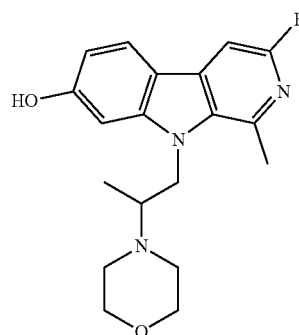
3-fluoro-1-methyl-9-(2-morpholinopropyl)-9H-pyrido[3,4-b]indol-7-ol;
