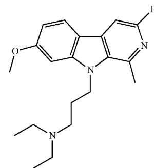
50 N,N-diethyl-3-(3-fluoro-7-methoxy-1-methyl-9H-pyrido[3,4-b]indol-9-yl)propan-1-amine;
