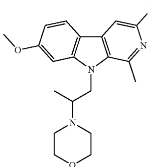
4-(1-(7-methoxy-1-methyl-9H-pyrido[3,4-b]indol-9-yl)propan-2-yl)morpholine;
