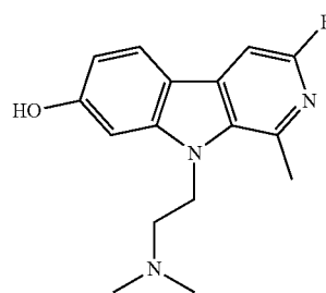
9-(2-(dimethylamino)ethyl)-3-fluoro-1-methyl-9H-pyrido[3,4-b]indol-7-ol;
