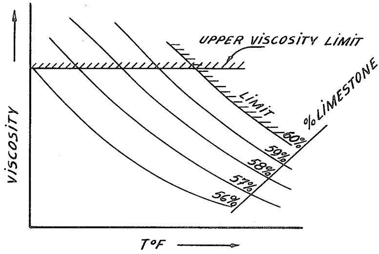
COATING MIXTURE VISCOSITY VS TEMP. % LIMESTONE
