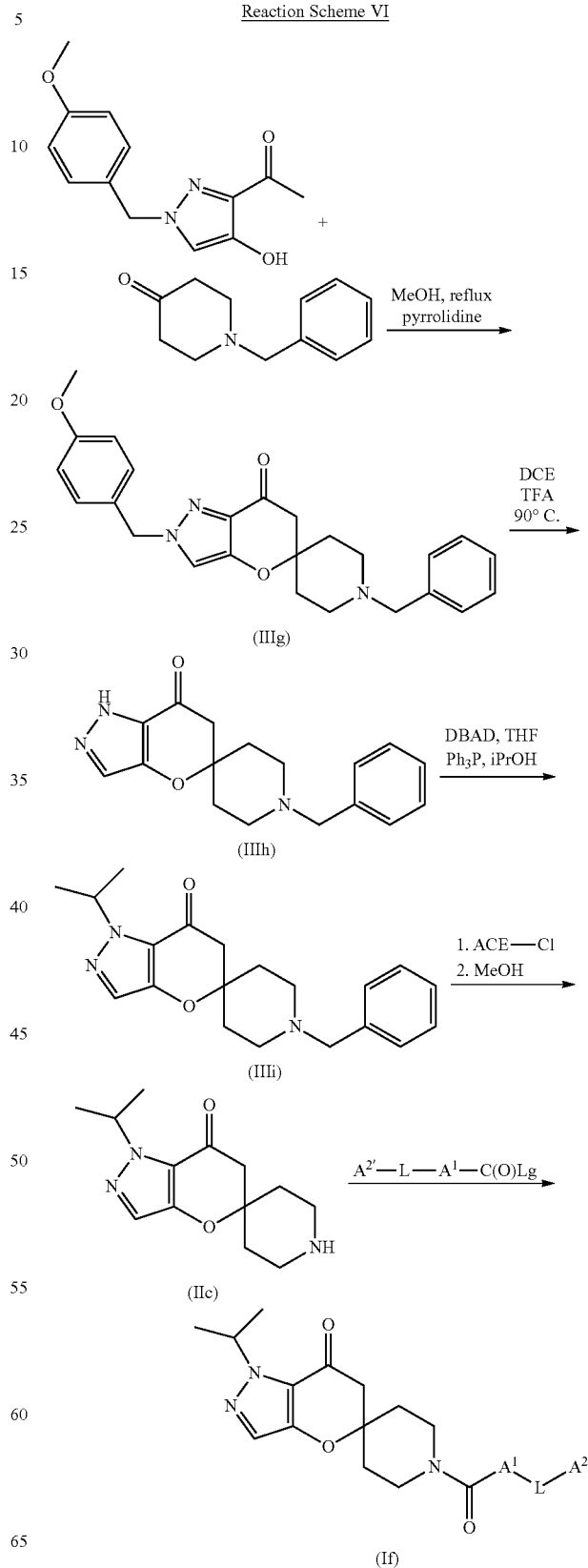
Reaction Scheme VI
