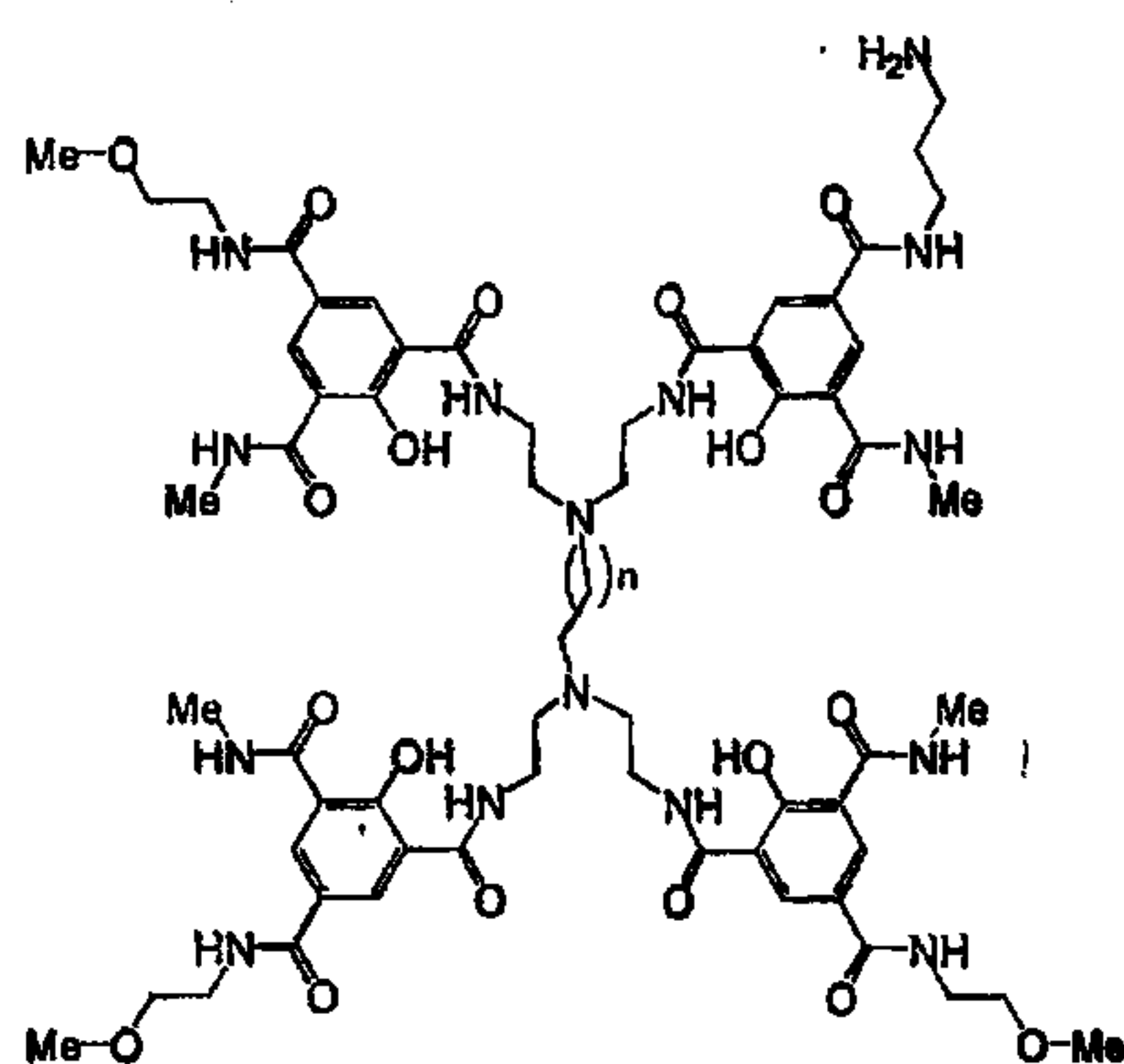
23A (n = 1)
