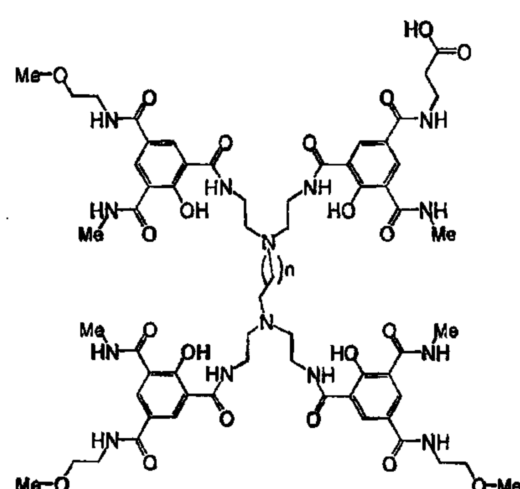
24A (n = 1)
