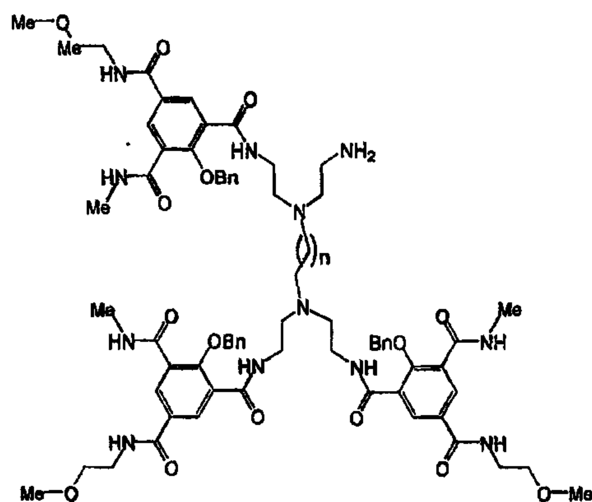
(22A, n = 1)
