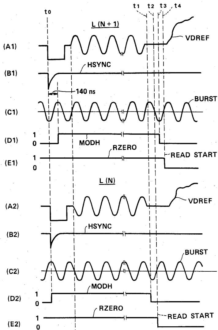
SIG. WAVEFORMS OF EACH SECTION IN FIG. 2
