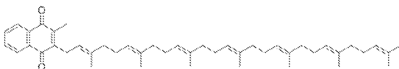
(Formula I).
