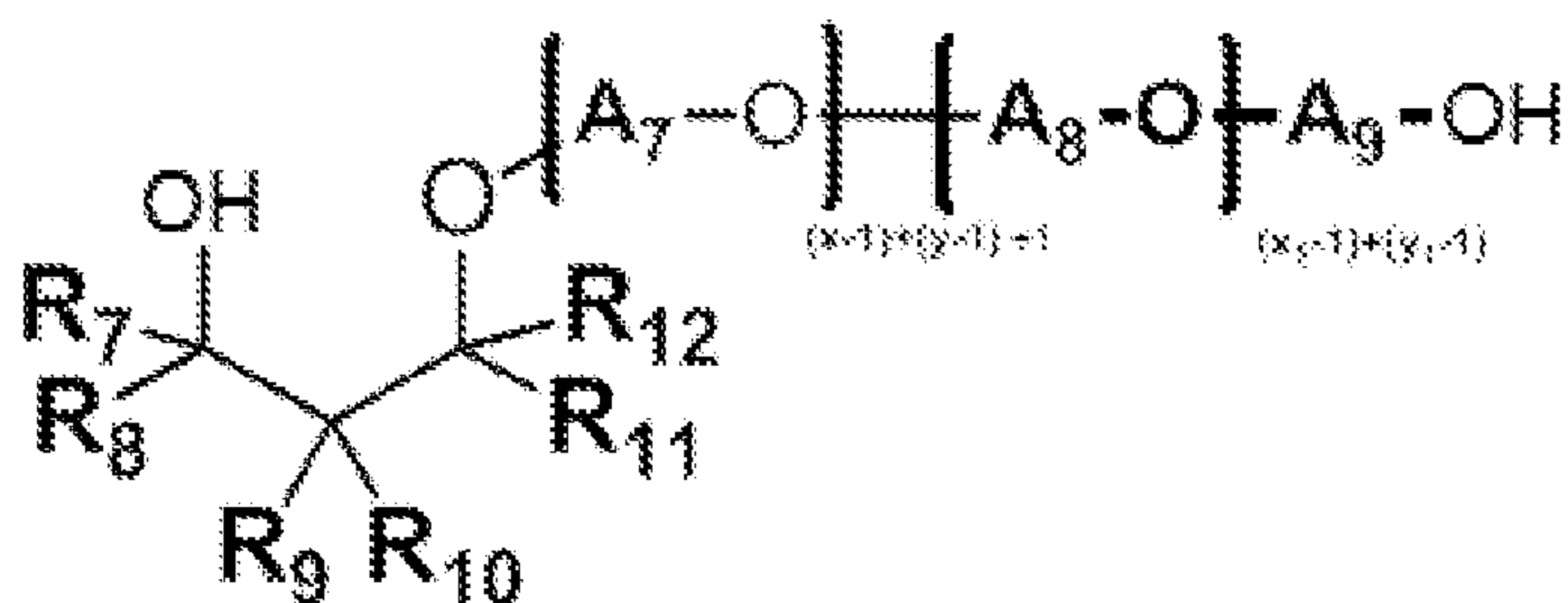
Formula (V)
