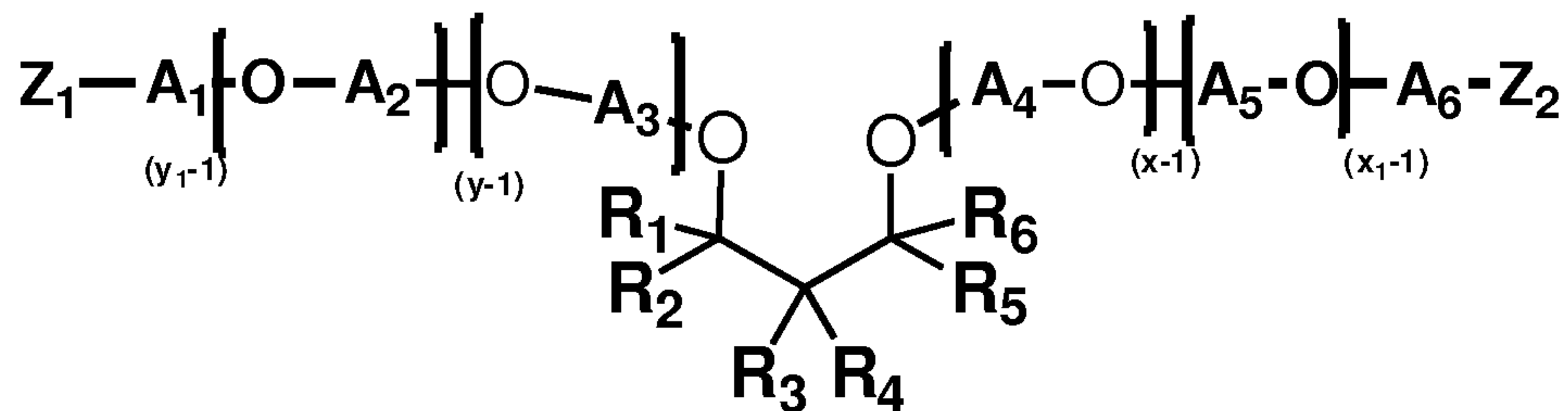
Formula I
