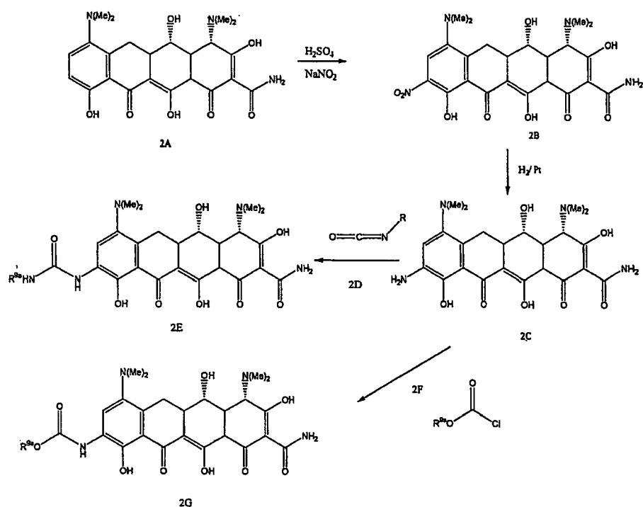
SCHEME 2
