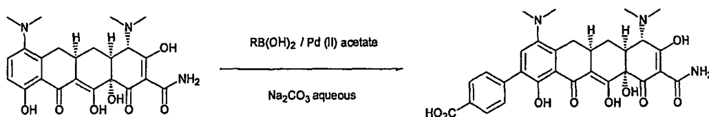
SCHEME 8
