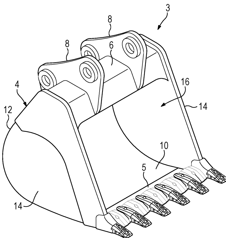
FIG. 2 Prior Art
