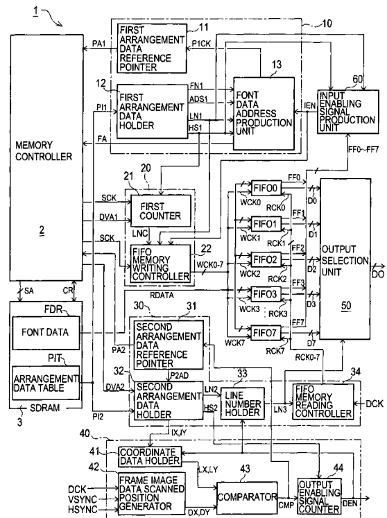
FIG. 1 CIRCUITRY OF IMAGE DISPLAY SYSTEM IN ACCORDANCE WITH PRESENT EMBODIMENT
