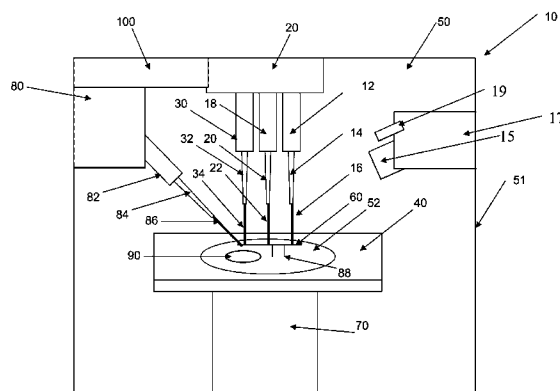
Diagram of Precision Fabrication System.
