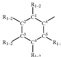
\beta -ionone Ring Structure
