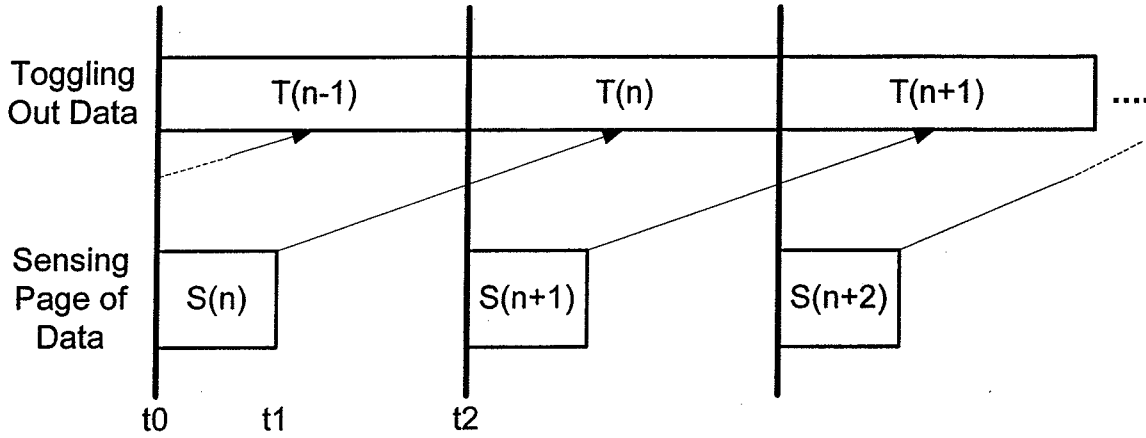
Conventional Read Caching FIG. 37
