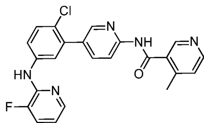
Compound 15
