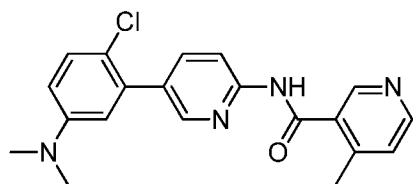
Compound 138
