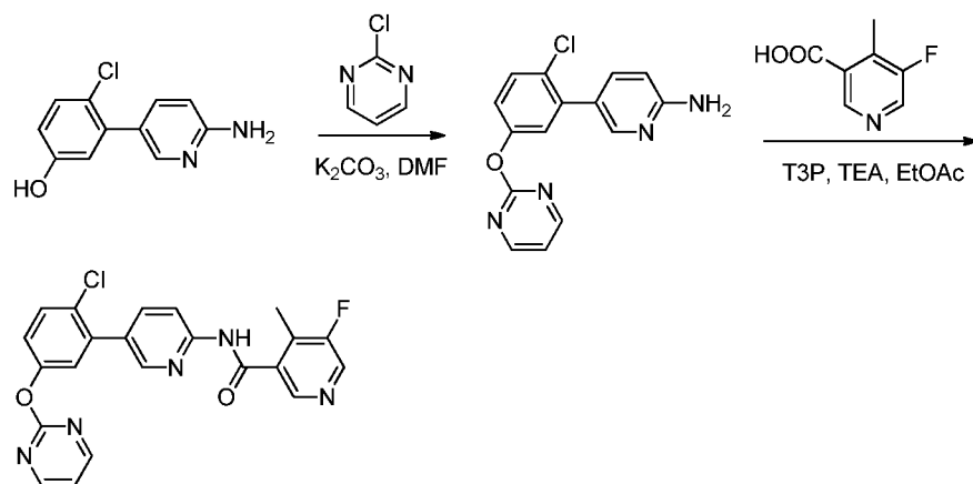
Compound 23
