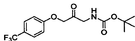
tert -butyl 2-oxo-3-(4-(trifluoromethyl)phenoxy)propylcarbamate
