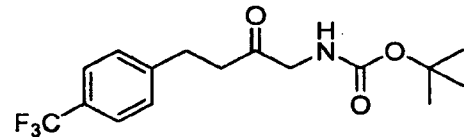
tert -butyl 2-oxo-4-(4-(trifluoromethyl)phenyl)butylcarbamate
