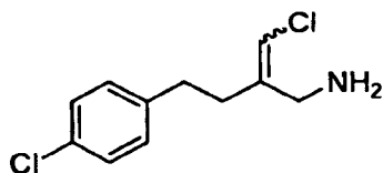
2-(chloromethylene)-4-(4-chlorophenyl)butan-1-amine
