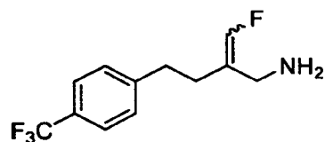
2-(fluoromethylene)-4-(4-(trifluoromethyl)phenyl)butan-1-amine
