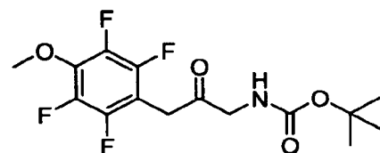
tert -butyl 2-oxo-3-(2,3,5,6-tetrafluoro-4-methoxyphenyl)propylcarbamate
