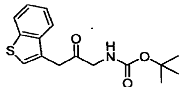
tert -butyl 3-(benzo[ b ]thiophen-3-yl)-2-oxopropylcarbamate
