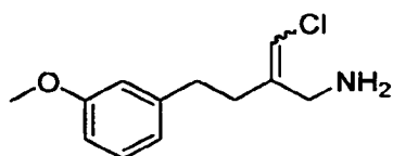
2-(chloromethylene)-4-(3-methoxyphenyl)butan-1-amine
