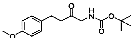
tert -butyl 4-(4-methoxyphenyl)-2-oxobutylcarbamate
