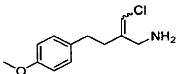
2-(chloromethylene)-4-(4-methoxyphenyl)butan-1-amine
