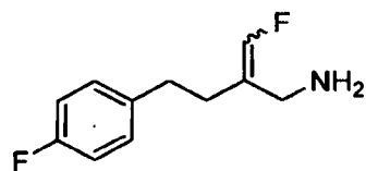
2-(fluoromethylene)-4-(4-fluorophenyl)butan-1-amine
