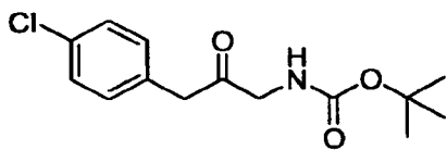
tert -butyl 3-(4-chlorophenyl)-2-oxopropylcarbamate
