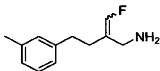
2-(fluoromethylene)-4- m -tolylbutan-1-amine
