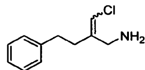
2-(chloromethylene)-4-phenylbutan-1-amine
