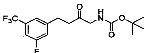
tert -butyl 4-(3-fluoro-5-(trifluoromethyl)phenyl)-2-oxobutylcarbamate
