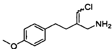
2-(chloromethylene)-4-(4-methoxyphenyl)butan-1-amine
