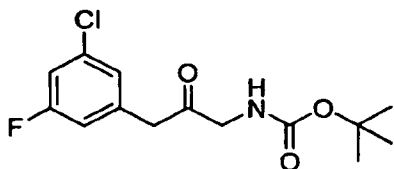
tert -butyl 3-(3-chloro-5-fluorophenyl)-2-oxopropylcarbamate
