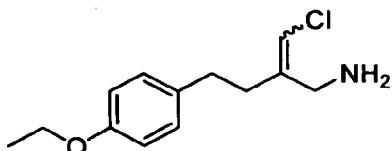
2-(chloromethylene)-4-(4-ethoxyphenyl)butan-1-amine
