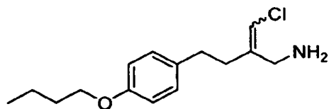
4-(4-butoxyphenyl)-2-(chloromethylene)butan-1-amine
