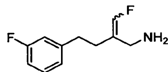
2-(fluoromethylene)-4-(3-fluorophenyl)butan-1-amine
