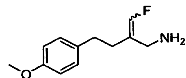
2-(fluoromethylene)-4-(4-methoxyphenyl)butan-1-amine
