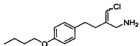
4-(4-butoxyphenyl)-2-(chloromethylene)butan-1-amine
