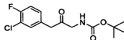
tert -butyl 3-(3-chloro-4-fluorophenyl)-2-oxopropylcarbamate
