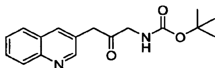
tert -butyl 2-oxo-3-(quinolin-3-yl)propylcarbamate
