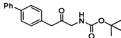
tert -butyl 3-(biphenyl-4-yl)-2-oxopropylcarbamate
