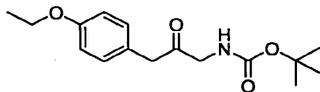
tert -butyl 3-(4-ethoxyphenyl)-2-oxopropylcarbamate
