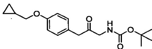
tert -butyl 3-(4-(cyclopropylmethoxy)phenyl)-2-oxopropylcarbamate
