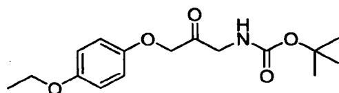
tert -butyl 3-(4-ethoxyphenoxy)-2-oxopropylcarbamate
