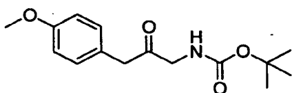
tert -butyl 3-(4-methoxyphenyl)-2-oxopropylcarbamate
