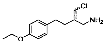
2-(chloromethylene)-4-(4-ethoxyphenyl)butan-1-amine
