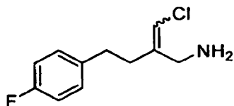
2-(chloromethylene)-4-(4-fluorophenyl)butan-1-amine
