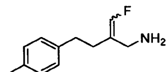
2-(fluoromethylene)-4- p -tolylbutan-1-amine
