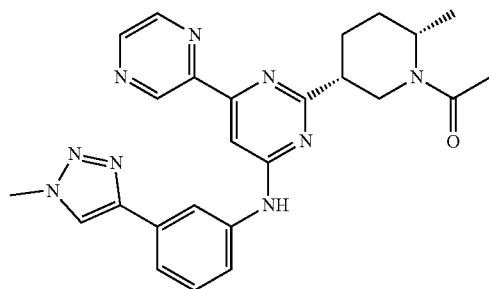
Compound C
