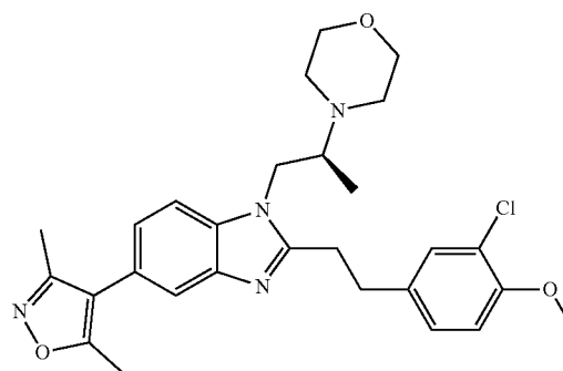
SGC-CBP30
