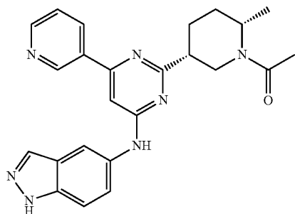
Compound 00030
