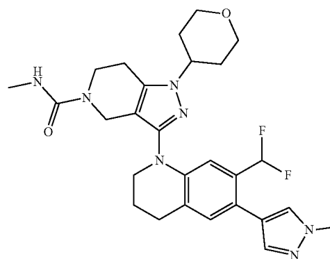
SGC-CBP30
