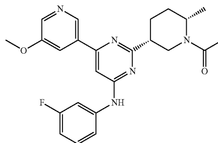
Compound A
