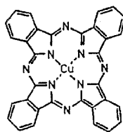
Cu-Phthalocyanine
