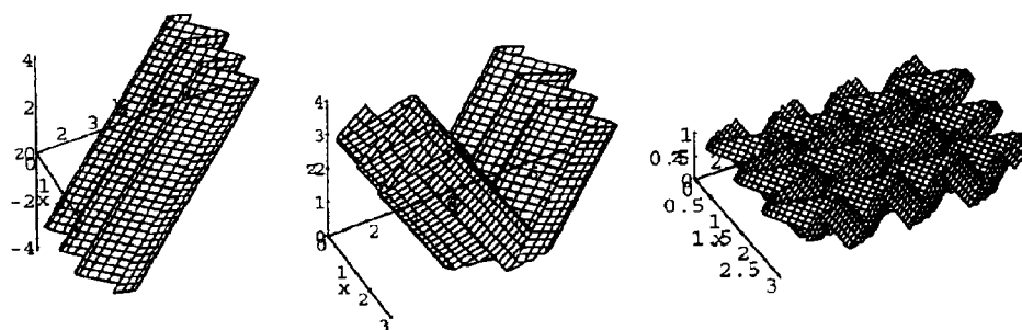
(a) \rho \circ (\gamma \times I)(\mathbb{R}^2) (b) (I \times I \times | \cdot |) \circ \rho \circ (\gamma \times I)(\mathbb{R}^2) (c) (I \times I \times \Xi) \circ \rho \circ (\gamma \times I)(\mathbb{R}^2)
