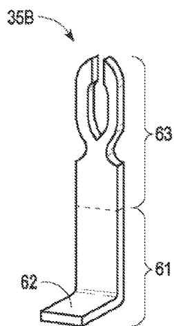
FORK ELECTRICAL PRESS-FIT TERMINAL
