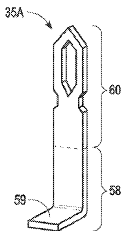
EYE-OF-THE-NEEDLE ELECTRICAL PRESS-FIT TERMINAL
