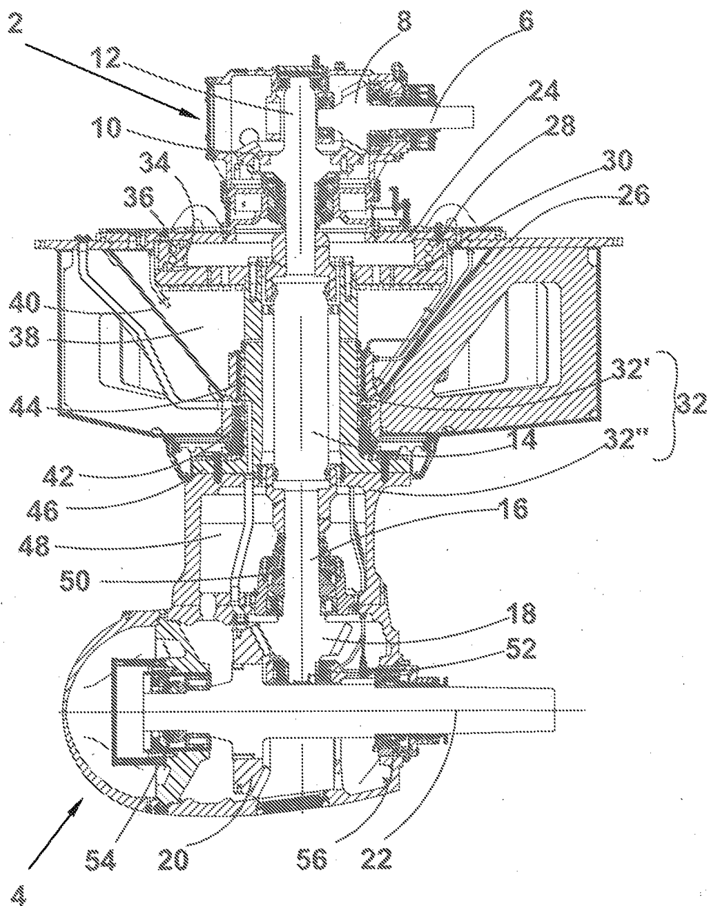
Fig. 1 (Prior Art)
