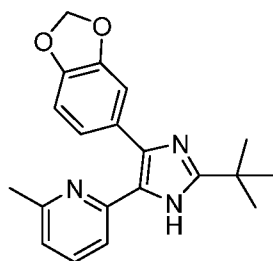
SB-505124
