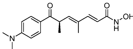
Trichostatin A
