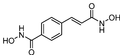
CBHA
