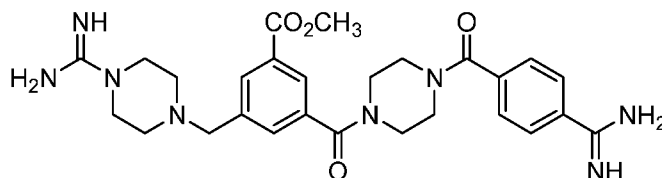
Formula IV
