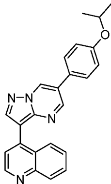
Formula XIII
