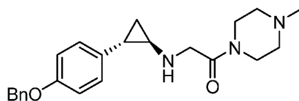
Formula II
