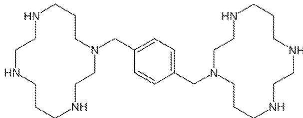
AMD3100
