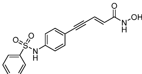
Oxamflatin
