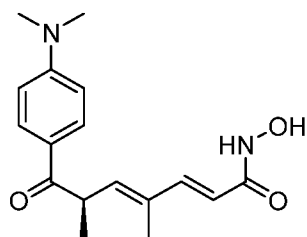
Formula IX
