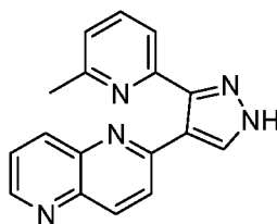
Formula VI
