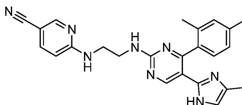
Formula XII
