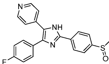
Formula VIII
