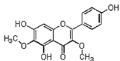
Compound 13
