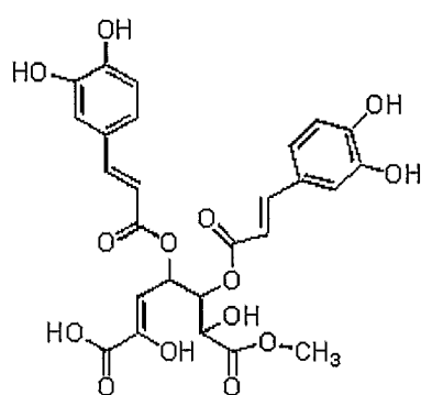
Compound 8
