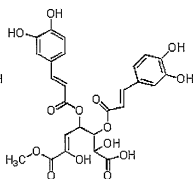
Compound 9
