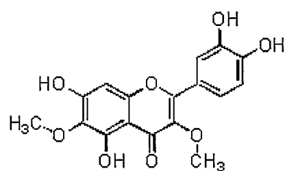
Compound 11
