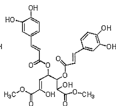
Compound 10
