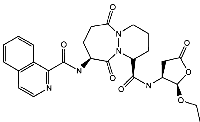
(compound 1);
