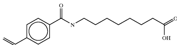
8-(vinylbenzoyl)aminocaproic acid
