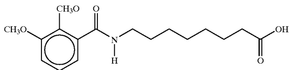
8-(N-2,3-Dimethoxybenzoyl)aminocaprylic acid
