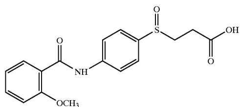
4-(2-methoxybenzoyl)amino 3-carboxysulfoxide
