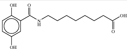
8-(N-2,5-Dihydroxybenzoyl)aminocaprylic acid
