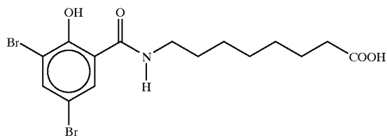
8-[N-(2-acetoxy-3,5-dibromobenzoyl)]aminocaprylic acid
