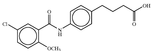
4-(4-(5-chloro-o-anisoyl)aminophenyl)butyric acid
