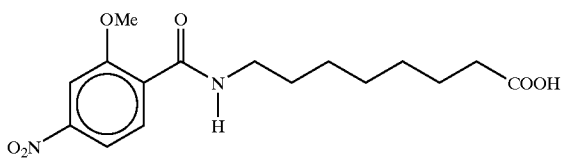
8-N-(2-methoxy-4-nitrobenzoyl)aminocaprylic acid
