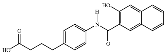
4-{4-[N-(3-hydroxy-2-naphthoyl)aminophenyl]}butyric acid
