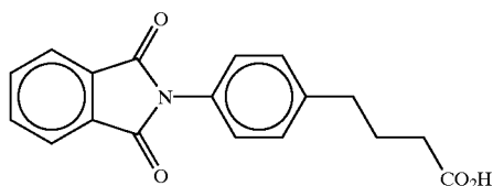
4-(4-phthalimidophenyl)butyric acid
