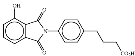
4-(4-(3-hydroxyphthalimido)phenyl)butyric acid
