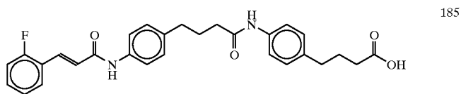
4-(4-(N-(2-Fluorocinnamoyl))aminophenyl) butyric
