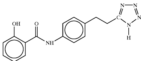
4-(Salicyloyl)aminophenylethyltetrazole
