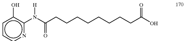
9-[2-(3-hydroxy)pyridylaminocarbonyl]nonanic acid
