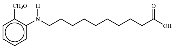
2-Methoxybenzenaminodecanoic acid
