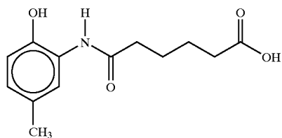
9-(2-hydroxy-5-methylanilincarbonyl)nonanoic acid
