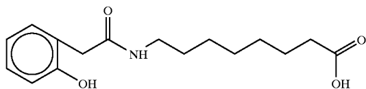
8-(2-hydroxyphenoxy)-aminocaprylic acid
