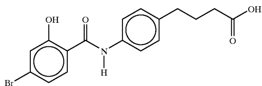
4-[N-(2-hydroxy-4-bromobenzoyl)aminophenyl]butyric acid
