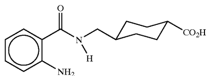
trans-4-(2-aminobenzamidomethyl)cyclohexanecarboxylic acid
