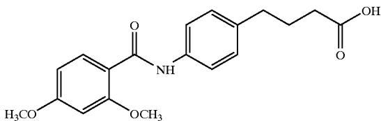
4-(4-(2,4-dimethoxybenzoyl)aminophenyl)butyric acid
