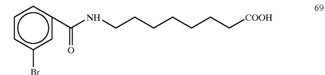
8-[N-(3-bromobenzoyl)]aminocaprylic acid
