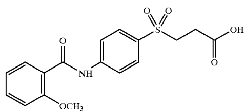
4-(2-methoxybenzoyl)amino 3-carboxysulfoxide
