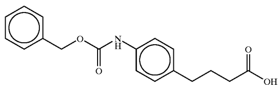
4-(4-benzyloxycarbonylamino)phenylbutyric acid
