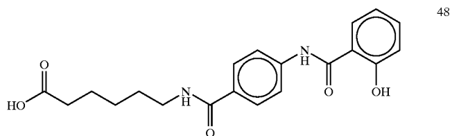
N-(4-salicyloylamino)-6-caproic acid
