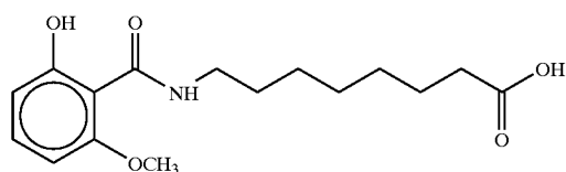
8-(N-(2-hydroxy-6-methoxybenzoyl)aminocaprylic acid
