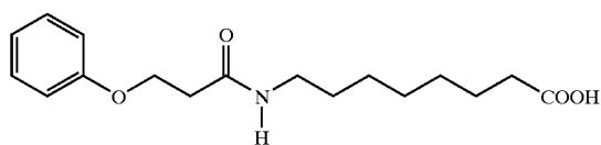
8-(3-Phenoxypropionylamino)caprylic acid
