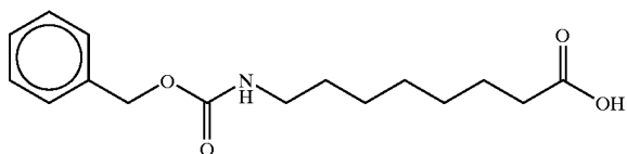
8-(Benzylcarbonylamino)caprylic acid
