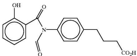
4-(4-(3-hydroxyphthalimido)phenyl)butyric acid
