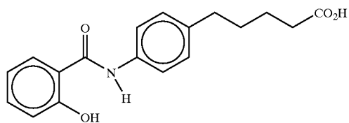
N-salicyloyl-5-(4-aminophenyl)valeric acid
