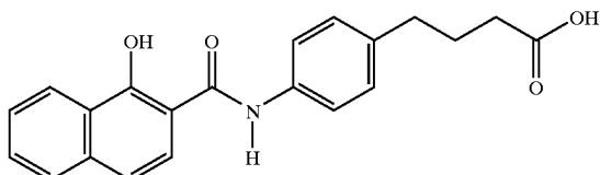
4-{4-[N-(1-hydroxy-2-naphthoyl)aminophenyl]}butyric acid
