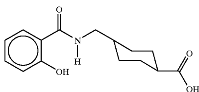
trans-4-(N-salicyloylaminomethyl)cyclohexanecarboxylic acid
