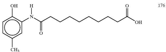
9-(2-hydroxy-5-methylanilino)nonanoic acid
