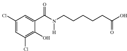
6-N-(3,5-dichloro-2-hydroxybenzoyl)aminocaproic acid
