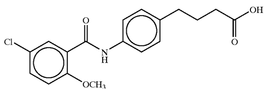
4-(4-(5-chloro-o-anisoyl)aminophenyl)butyric acid
