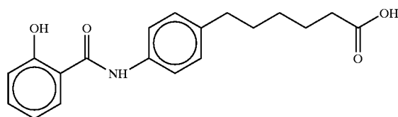
6-(4-(salicyloyl)aminophenyl)hexanoic acid
