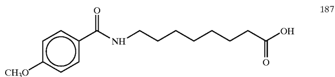
8-(p-anisoyl)aminocaprylic acid
