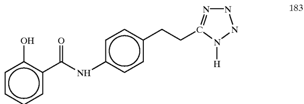
4-(salicyloyl)aminophenylethyltetrazole
