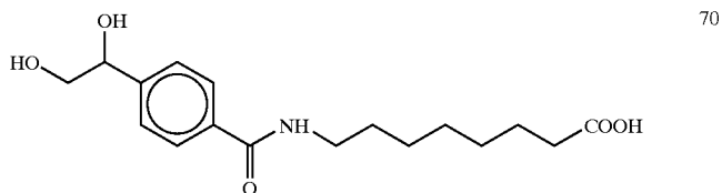
8-(4-(1,2-dihydroxyethyl)benzoyl)aminocaprylic acid
