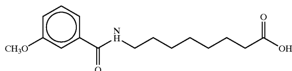
8-(3-anisoyl)aminocaprylic acid
