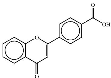
4'-flavonic acid
