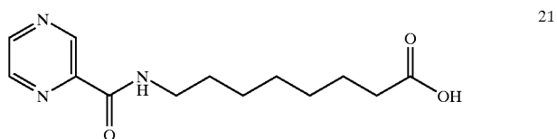
8-(2-pyrazinecarbonyl)aminocaprylic acid
