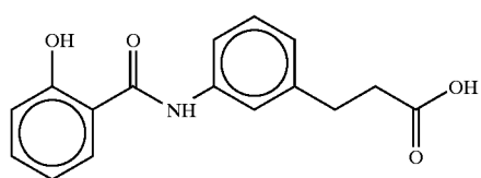
3-(3-(salicyloyl)aminophenyl)propionic acid
