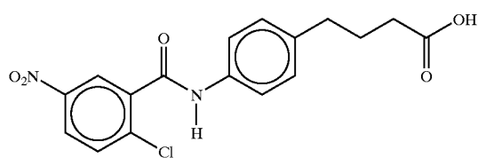
4-(4-(2-chloro-5-nitrobenzoyl)aminophenyl)butyric acid
