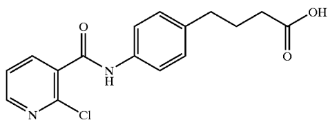
4-(4-(2-chloronicotinoyl)aminophenyl)butyric acid
