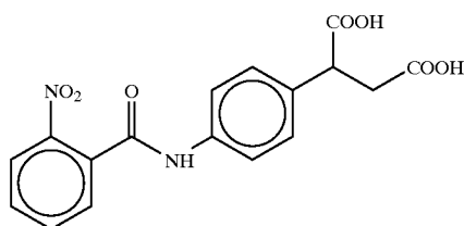
4(2-Nitrobenzoyl)aminophenylsuccinic acid
