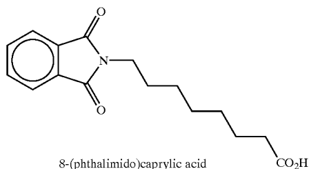
8-(phthalimido)caprylic acid
