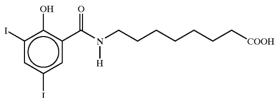
8-(N-2-hydroxy-3,5-diiodobenzoyl)aminocaprylic acid
