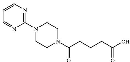
4-(1-(2-pyrimidinyl)piperazinoyl)butyric acid
