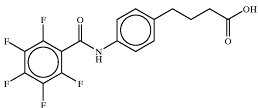
4-(4-pentafluorobenzoyl)aminophenyl)butyric acid
