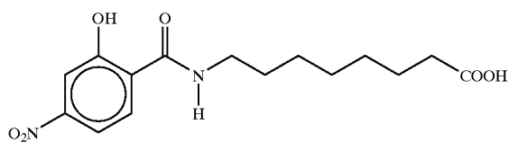
8-(N-2-hydroxy-4-nitrobenzoyl)aminocaprylic acid
