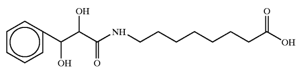
(3-phenyl-2,3-dihydroxypropanoyl)aminocaproic acid
