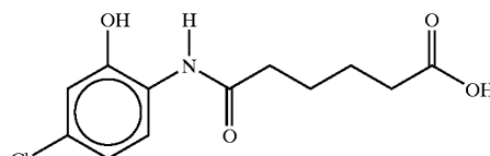
5-(4-chloro-2-hydroxyanilino)carbonyl]valeric acid
