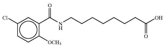
8-(5-chloro-o-anisoyl)aminocaprylic acid
