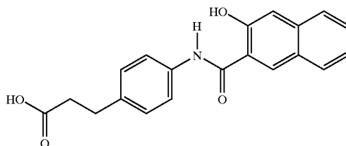
4-{4-[N-(3-hydroxy-2-naphthoyl)aminophenyl]}propanoic acid
