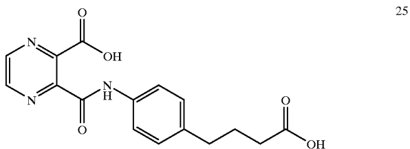
4-(4-(2-(3-carboxyl)pyrazinecarbonyl)aminophenyl)butyric acid
