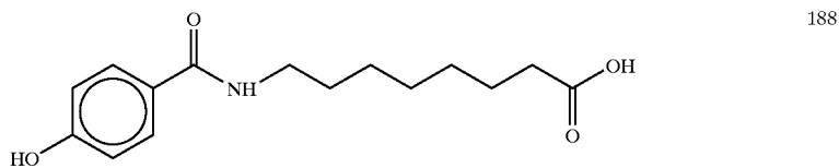
8-(4-Hydroxybenzoyl)aminocaprylic acid
