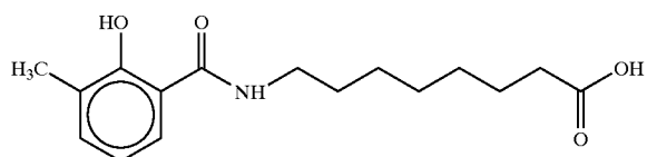
8-(N-(3-methylsalicyloyl)aminocaprylic acid
