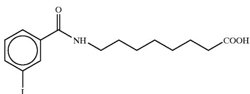
8-N-(3-iodobenzoyl)aminocaprylic acid
