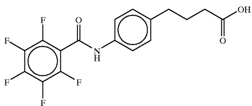
4-(4-pentafluorobenzoyl)aminophenyl)butyric acid
