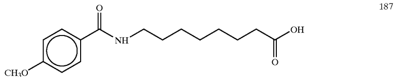
8-(p-anisoyl)aminocaprylic acid
