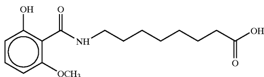
8-(N-2-Hydroxy-6-methoxybenzoyl)aminocaprylic acid
