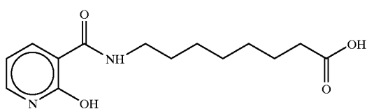
8-(2-Hydroxynicotinoyl)aminocaprylic acid
