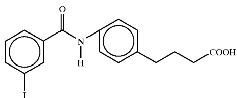
4-[N-[4-(3-iodobenzoyl)aminophenyl]]butyric acid
