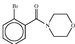
N-(2-bromobenzoyl)morpholine
