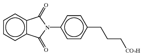
4-(4-phthalimidophenyl)butyric acid
