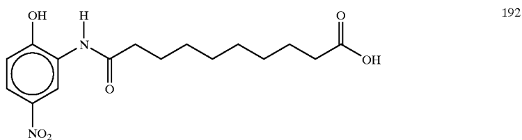
N-10-(2-hydroxy-5-nitroanilino)decanoic acid
