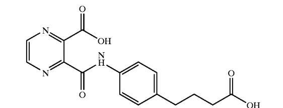
4-(4-(2-(3-carboxyl)pyrazinecarboxyl)aminophenyl)butyric acid
