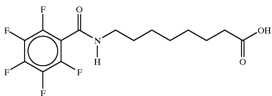
8-(pentafluorobenzoyl)aminocaprylic acid
