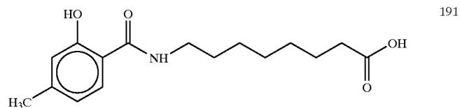
8-(N-4-Methylsalicyloyl)aminocaprillic acid[sic]
