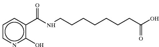
8-(2-Hydroxynicotinoyl)aminocaprylic acid
