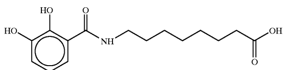
8-(N-(2,3-Dihydroxybenzoyl)aminocaprylic acid
