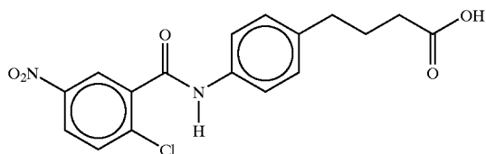
4-(4-(2-chloro-5-nitrobenzoyl)aminophenyl)butyric acid
