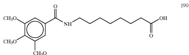
8-(3,4,5-Trimethoxybenzoyl)aminocaprylic acid
