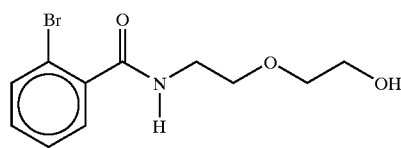
2-[N-(2-bromobenzoyl)aminoethoxy]ethanol
