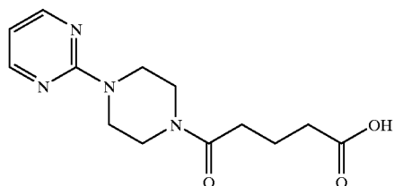
4-(1-(2-pyrimidyl)piperazinyl)butyric acid
