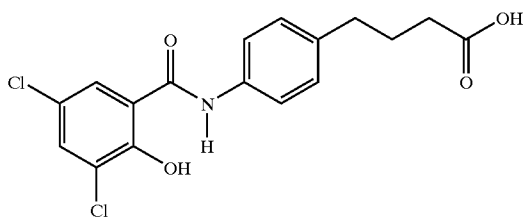
N-[3,5-dichloro-2-hydroxybenzoyl]-4-(4-aminophenyl)butyric acid
