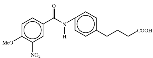
4-[N-(4-(4-methoxy-3-nitrobenzoyl)aminophenyl)]butyric acid
