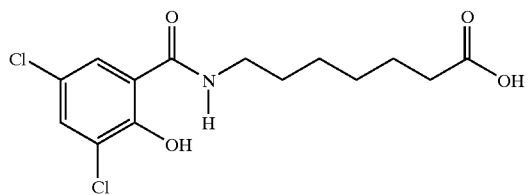
7-N-(3,5-dichloro-2-hydroxybenzoyl)aminoheptanoic acid
