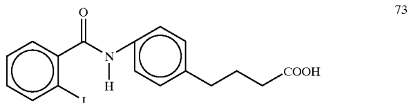
4-{4-[N-(2-iodoenzoyl)aminophenyl]}butyric acid
