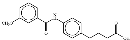
4-(4-(3-anisoyl)aminophenyl)butyric acid
