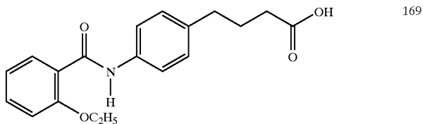
4-(4-(2-ethoxybenzoyl)aminophenyl)butyric acid
