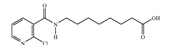
8-(2-chloronicotinoyl)aminocaprylic acid
