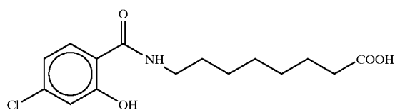
8-(2-hydroxy-4-chlorobenzoyl)aminocaprylic acid
