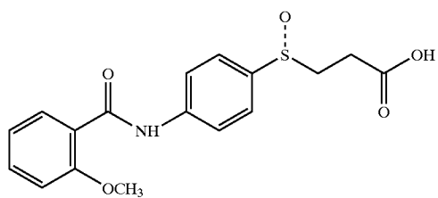
4-(2-methoxybenzoyl)amino 3-carboxysulfoxide
