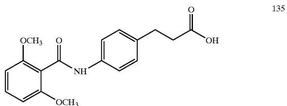
3-(4-(2,6-dimethoxybenzoyl)aminophenyl)propionic acid
