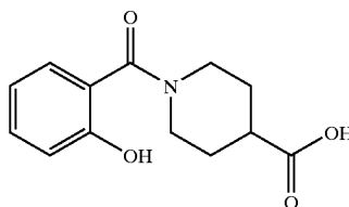
N-(2-hydroxybenzoyl)isonipecotic acid
