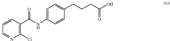
4-(4-(2-chloronicotinoyl)aminophenyl)butyric acid
