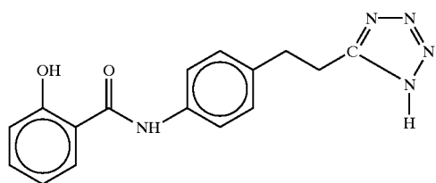
4-(Salicyloyl)aminophenylethyltetrazole
