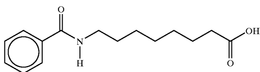
8-(N-benzoyl)aminocaprylic acid
