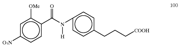
4-{N-[4-(2-methoxy-2-nitrobenzoyl)aminophenyl]}butyric acid
