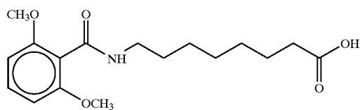
8-(N-(2,6-Dimethoxybenzoyl)aminocaprylic acid
