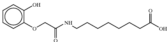
7-(2-hydroxyphenoxy)acetyl)aminocaprylic acid
