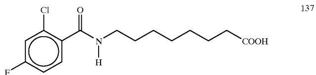
8-(N-(2-chloro-4-fluorobenzoyl)aminocaprylic acid
