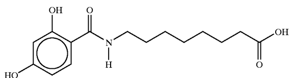
8-(N-2,4-Dihydroxybenzoyl)aminocaprylic acid
