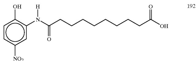
N-10-(2-hydroxy-5-nitroanilino)decanoic acid
