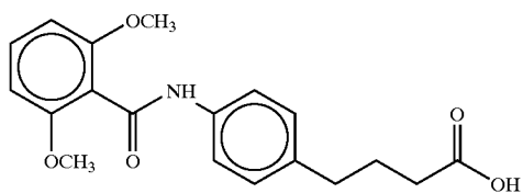
4-(4-(2,6-dimethoxybenzoyl)aminophenyl)butyric acid
