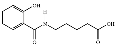
5-(N-salicyloylamino)valeric acid
