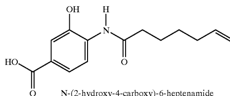
N-(2-hydroxy-4-carboxy)-6-heptenamide
