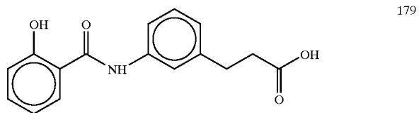
3-(3-(salicyloyl)aminophenyl)propionic acid
