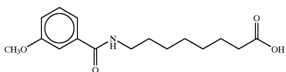
8-(3-anisoyl)aminocaprylic acid
