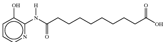
9-[2-(3-hydroxy)pyridylaminocarbonyl]nonanoic acid
