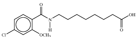
8-(4-chloro-o-anisoyl)aminocaprylic acid
