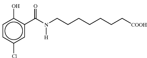
8-(N-(2-hydroxy-5-chlorobenzoyl)aminocaprylic acid
