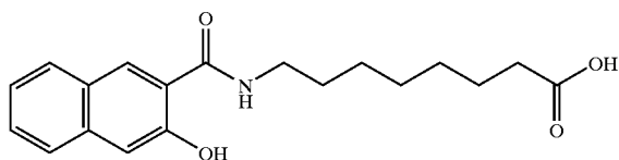
8-(3-hydroxy-2-naphthoyl)aminocaprylic acid
