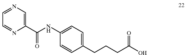
4-(4-(2-pyrazinecarbonyl)aminophenyl)butyric acid
