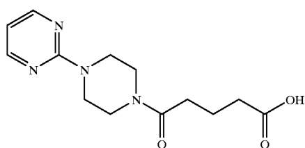
4-(1-(2-pyrimidyl)piperazinoyl)butyric acid
