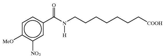
8-N-(4-methoxy-3-nitrobenzoyl)aminocaprylic acid
