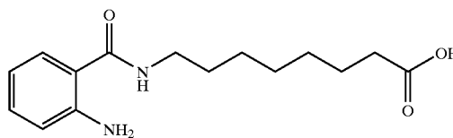
8(2-aminobenzoylamino)caprylic acid
