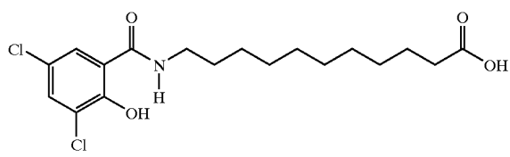
11-N-(3,5-dichloro-2-hydroxybenzoyl)aminoundecanoic acid
