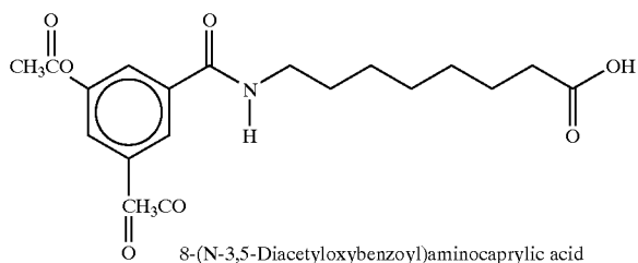
8-(N-3,5-Diacetyloxybenzoyl)aminocaprylic acid
