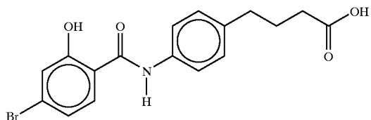
4-[N-(2-hydroxy-4-bromobenzoyl)aminophenyl]butyric acid
