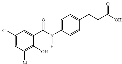
N-[3,5-dichloro-2-hydroxybenzoyl-3-(4-aminophenyl)]propionic acid
