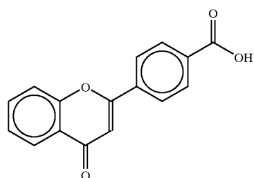
4'-flavonic acid
