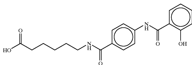
N-(4-salicyloylamino)-6-caproic acid
