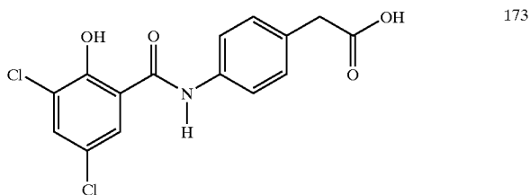
4-[N-(3,5-dichloro-2-hydroxybenzoyl)aminophenyl]acetic acid
