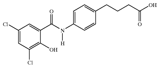
N-[3,5-dichloro-2-hydroxybenzoyl]-4-(4-aminophenyl)butyric acid
