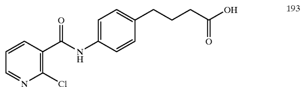
4-(4-(2-chloronicotinoyl)aminophenyl)butyric acid
