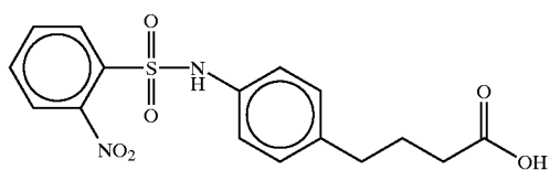
4-(4-(2-nitrobenzenesulfonyl)aminophenyl)butyric acid
