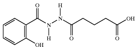
1-salicyloyl-2-glutaryl hydrazide
