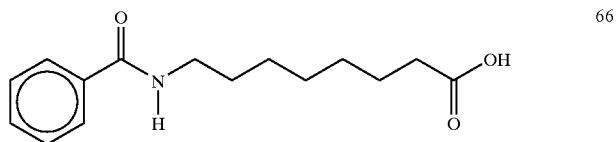
8-(N-benzoyl)aminocaprylic acid
