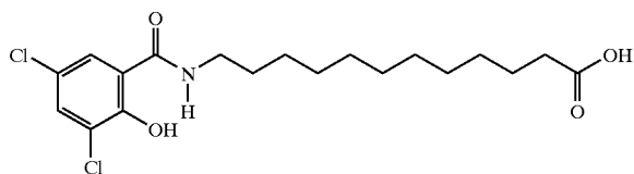
12-N-(3,5-dichloro-2-hydroxybenzoyl)aminododecanoic acid
