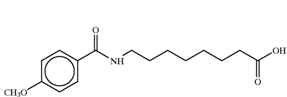
8-(p-anisoyl)aminocaprylic acid
