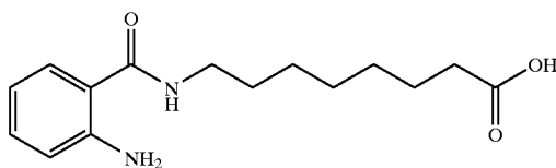
8(2-aminobenzoylamino)caprylic acid
