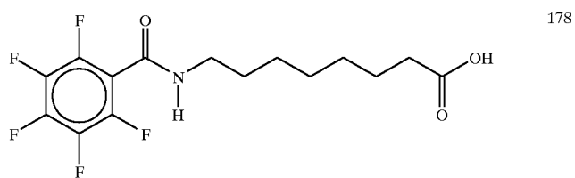
8-(pentafluorobenzoyl)aminocaproic acid
