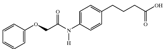
4-(4-(phenoxyacetyl)aminophenyl)butyric acid
