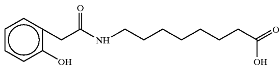
8-(2-hydroxyphenoxy)aminocaproic acid
