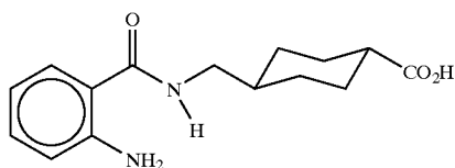
trans-4-(2-aminobenzamidomethyl)cyclohexanecarboxylic acid
