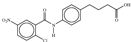
4-(4-(2-chloro-5-nitrobenzoyl)aminophenyl)butyric acid
