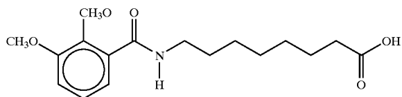
8-(N-(2,3-Dimethoxybenzoyl)]aminocaprylic acid
