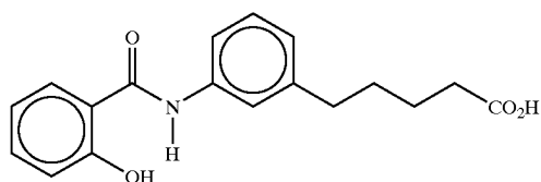
N-salicyl-5-(3-aminophenyl)valeric acid
