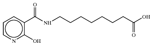
8-(2-Hydroxynicotinoyl)aminocaproic acid
