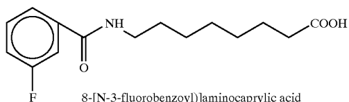
8-[N-(3-fluorobenzoyl)]aminocaproic acid
