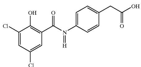
4-[N-(3,5-dichloro-2-hydroxybenzoyl)]aminophenylacetic acid
