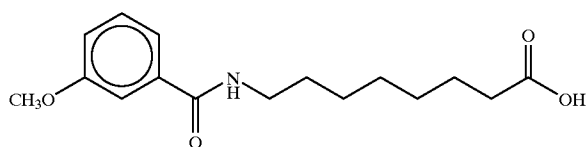
8-(3-anisoyl)aminocaprylic acid
