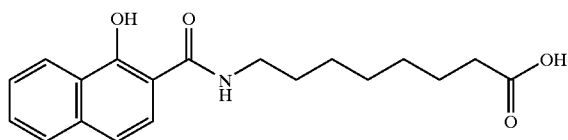
8-(N-1-hydroxy-2-naphthoyl)aminocaprylic acid
