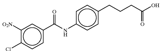
4-(4-(4-chloro-3-nitrobenzoyl)aminophenyl)butyric acid
