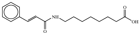
8-cinnamoylaminovaleric acid
