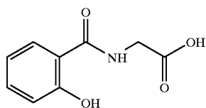
salicyloylglycine
