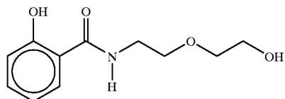
2-[N-(2-hydroxybenzoylamino)ethoxy]ethanol
