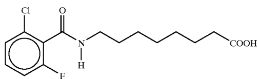
8-N-(2-chloro-6-fluorobenzoyl)aminocaprylic acid
