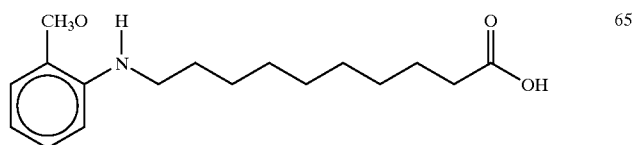
2-Methoxybenzenaminodecanoic acid
