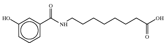
8-(3-Hydroxybenzoyl)aminocaprylic acid
