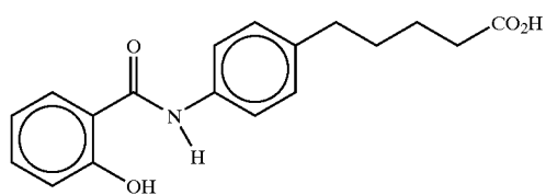
N-salicyl-5-(4-aminophenyl)valeric acid
