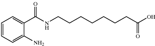
8(2-aminobenzoylamino)caprylic acid
