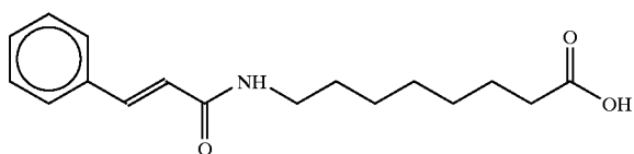
8-cinnamoylaminocaprylic acid
