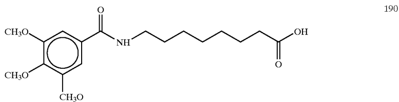
8-(3,4,5-Trimethoxybenzoyl)aminocaprylic acid
