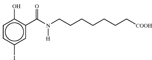
8-(N-(2-hydroxy-5-iodobenzoyl)aminocaprylic acid
