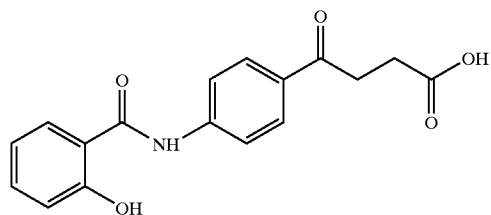
4-(4-Salicyloylaminophenyl)-4-oxobutyrlic acid
