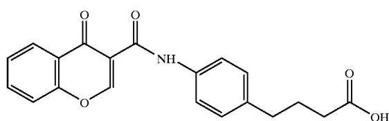
4-(4-(chromone-3-carbonyl)aminophenyl)butyric acid
