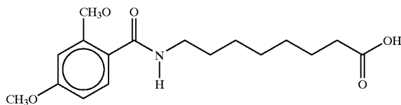
8-(N-2,4-Dihydroxybenzoyl)aminocaprylic acid
