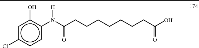
8-(2-hydroxy-5-chloroanilino)octanoic acid
