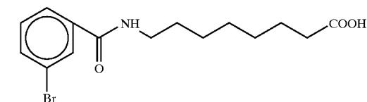
8-[N-(3-bromobenzoyl)]aminocaprylic acid
