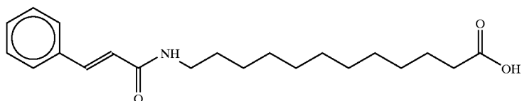
12-cinnamoyldodecanoic acid
