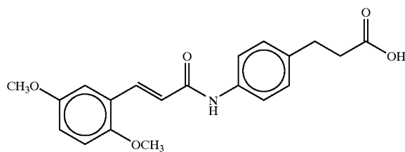
3-(4-(2,5-dimethoxycinnamoyl)aminophenyl)propionic acid
