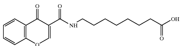
8-(chromone-3-carbonyl)aminocaproic acid
