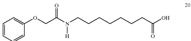
8-(Phenoxyacetylamino)caprylic acid
