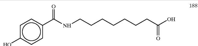
8-(4-Hydroxybenzoyl)aminocaprylic acid
