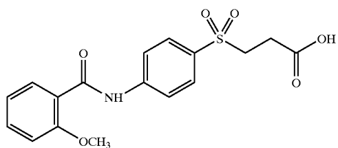
4-(2-methoxybenzoyl)amino 3-carboxypropylsulfone
