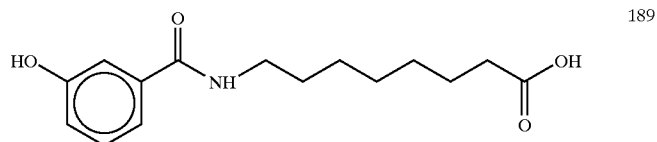
8-(3-Hydroxybenzoyl)aminocaprylic acid
