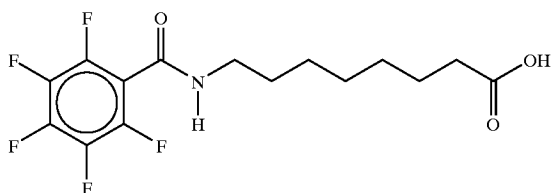
8-(pentafluorobenzoyl)aminocaprylic acid
