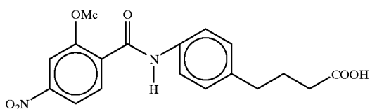
4-[N-(4-(2-methoxy-4-nitrobenzoyl)aminophenyl)]butyric acid
