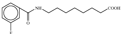
8-[N-(3-fluorobenzoyl)]aminocaprylic acid
