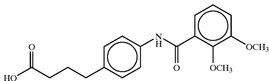
4-(2-(2,3-dimethoxybenzoyl)aminophenyl)butyric acid
