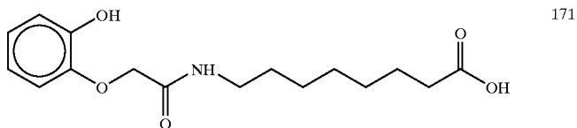
7-(2-hydroxyphenoxyacetyl)aminocaprylic acid
