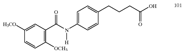
4-(4-(2,5-dimethoxybenzoyl)aminophenyl)butyric acid
