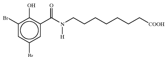
8-[N-(2-acetoxy-3,5-dibromobenzoyl)]aminocaprylic acid
