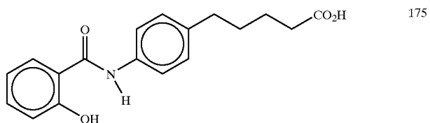
N-salicyl-5-(4-aminophenyl)valeric acid
