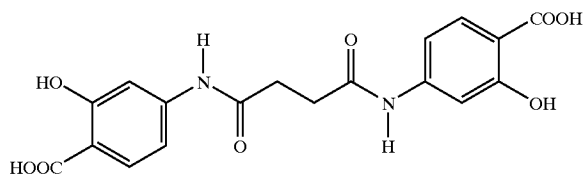
Succinyl-4-aminosalicylic acid
