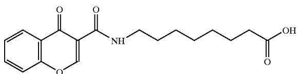
8-(chromone-3-carbonyl)aminocaprylic acid
