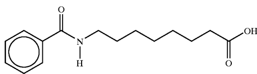
8-(N-benzoyl)aminocaprylic acid
