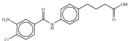
4-(4-(4-chloro-3-nitrobenzoyl)aminophenyl)butyric acid
