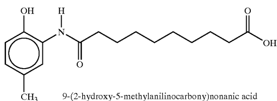
9-(2-hydroxy-5-methylanilincarbonyl)nonanoic acid
