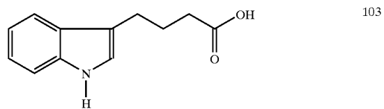
3-Indolebutyric acid
