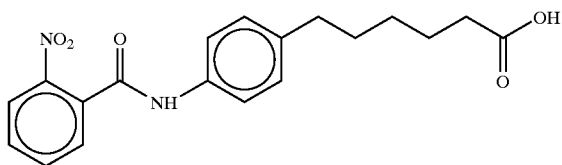
6-(4-(N-2-Nitrobenzoyl)aminophenyl)hexanoic acid
