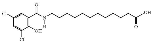
12-N-(3,5-dichloro-2-hydroxybenzoyl)aminododecanoic acid
