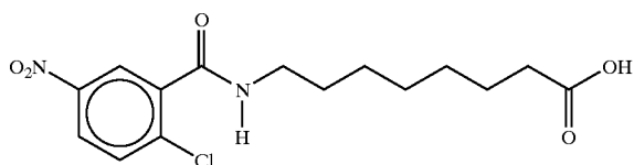
8-(2-chloro-5-nitrobenzoyl)aminocaprylic acid
