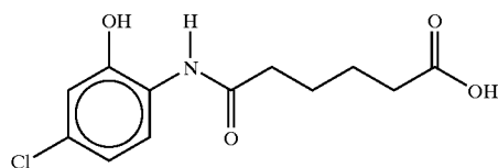
5-(4-chloro-2-hydroxyanilino)valeric acid
