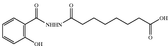
1-salicyloyl-2-suberyl hydrazide
