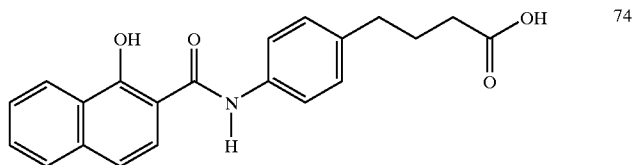
4-{4-[N-(1-hydroxy-2-naphthoyl)aminophenyl]}butyric acid
