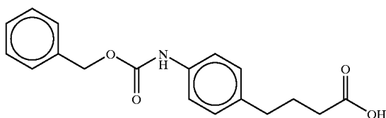
4-(4-benzoyloxycarbonylamino)phenyl)butyric acid
