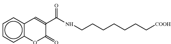
8-[N-(3-coumarincarbonyl)]aminocaproic acid
