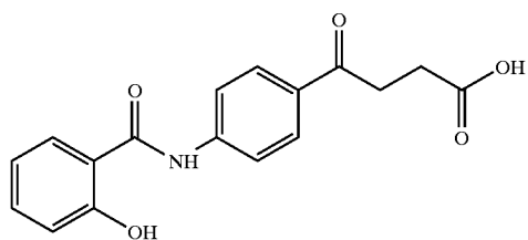
4-(4-(4-salicyloylaminophenyl)-4-oxobutyl)butyric acid
