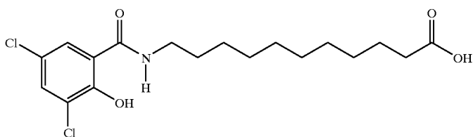
11-N-(3,5-dichloro-2-hydroxybenzoyl)aminoundecanoic acid
