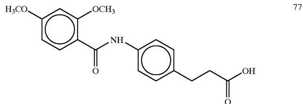
3-[4-(2,4-dimethoxybenzoyl)aminophenyl]propionic acid
