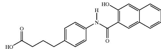
4-{4-[N-(3-hydroxy-2-naphthoyl)aminophenyl]}butyric acid
