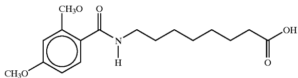
8-(N-(2,4-Dihydroxybenzoyl)]aminocaprylic acid
