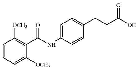
3-(4-(2,6-dimethoxybenzoyl)aminophenyl)propionic acid
