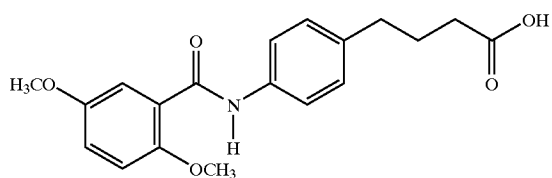
4-(4-(2,5-dimethoxybenzoyl)aminophenyl)butyric acid
