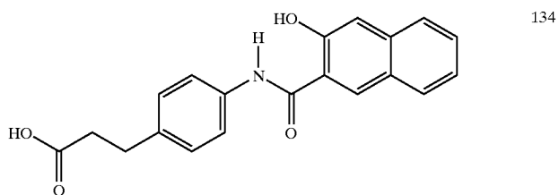
4-[4-[N-(3-hydroxy-2-naphthoyl)aminophenyl]]propanoic acid
