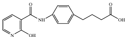
4-(4-(2-hydroxynicotinoyl)aminophenyl)butyric acid
