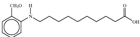
2-Methoxybenzenaminodecanoic acid
