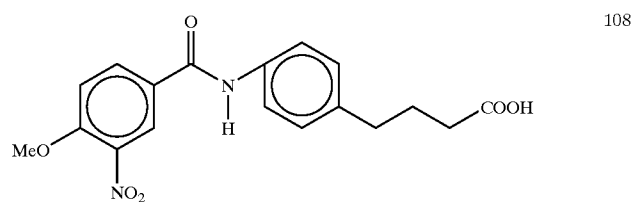
4-[4-N-(4-methoxy-3-nitrobenzoyl)aminophenyl]butyric acid
