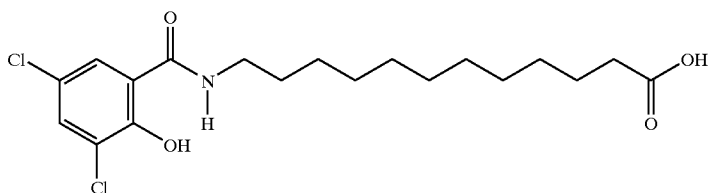
12-N-(3,5-dichloro-2-hydroxybenzoyl)aminododecanoic acid
