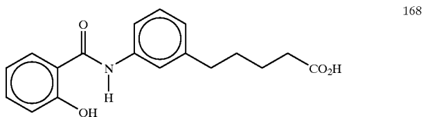
N-Salicoyl-5-(3-aminophenyl)valeric acid
