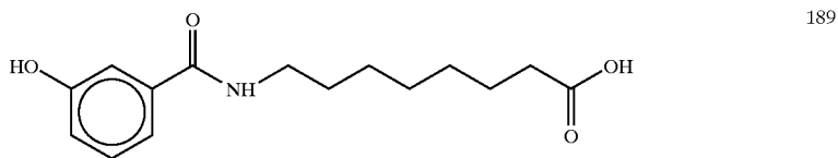
8-(3-Hydroxybenzoyl)aminocaprylic acid
