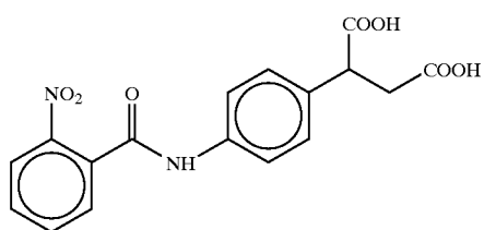
4-(2-Nitrobenzoyl)aminophenylsuccinic acid
