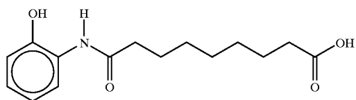
9-(2-hydroxybenzamido)nonanic acid
