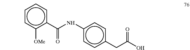
4-(o-anisoyl)aminophenylacetic acid
