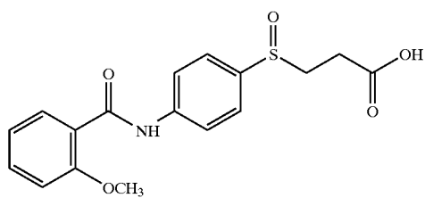
4-(2-methoxybenzoyl)amino 3-carboxysulfoxide
