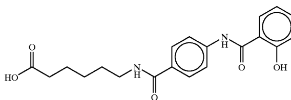
N-(4-salicyloylamino)-6-caproic acid
