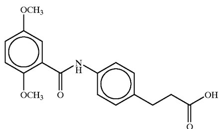
3-(4-(2,5-dimethoxybenzoyl)aminophenyl)propionic acid
