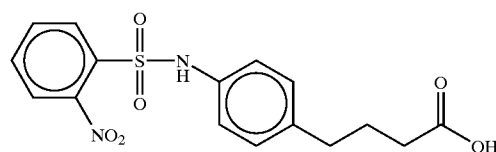
4-(4-(2-nitrobenzenesulfonyl)aminophenyl)butyric acid
