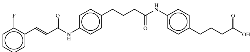
4-(4-(N-(2-Fluorocinnamoyl)aminophenyl)butyric)aminocaprylic acid
