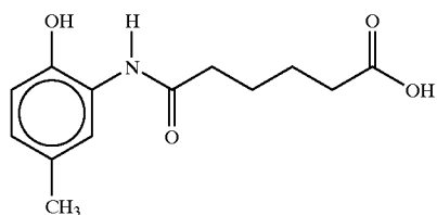
5-(2-hydroxy-5-methylanilincarbonyl)valeric acid
