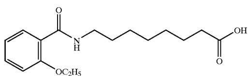
8-(2-ethoxybenzoyl)aminocaprylic acid
