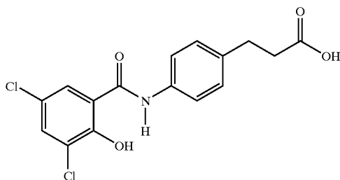
N-[3,5-dichloro-2-hydroxybenzoyl-3(4-aminophenyl)]propionic acid
