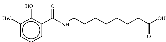
8-(N-(3-methylsalicyloyl)aminocaprylic acid
