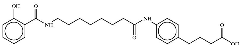
4-(4-(N-8(N-Salicyloyl)aminocaprylic)aminophenyl)butyric acid
