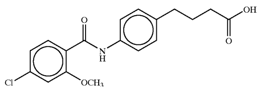
4-(4-(4-chloro-o-anisoyl)aminophenyl)butyric acid
