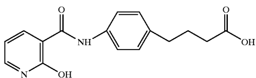
4-(4-(2-hydroxynicotinoyl)aminophenyl)butyric acid
