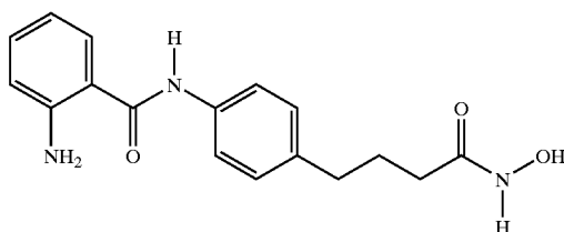
4-[4-(2-aminobenzoylamino)phenyl]butyrylhydroxamic acid
