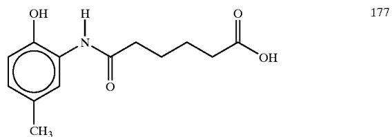
5-(2-hydroxy-5-methylanilino)valeric acid
