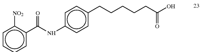
6-(4-(N-2-Nitrobenzoyl)aminophenyl)hexanoic acid
