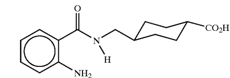
trans-4-(2-aminobenzamidomethyl)cyclohexanecarboxylic acid
