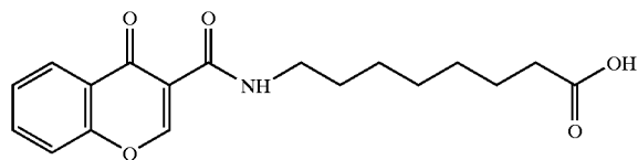
8-(chromone-3-carbonyl)aminocaproic acid
