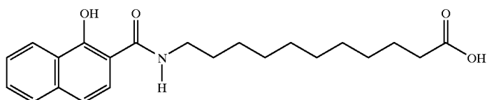
11-N-(1-hydroxy-2-naphthoyl)aminoundecanoic acid
