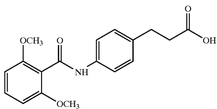
3-(4-(2,6-dimethoxybenzoyl)aminophenyl)propionic acid
