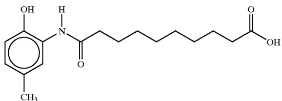
9-(2-hydroxy-5-methylanilincarbonyl)nonanoic acid
