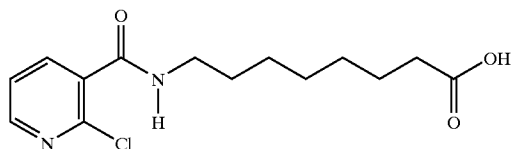
8-(2-chloronicotinoyl)aminocaprylic acid
