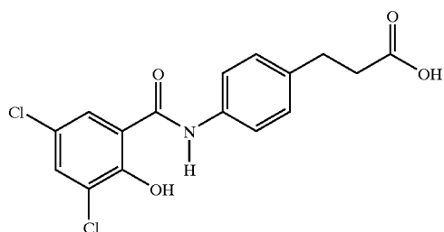
N-[3,5-dichloro-2-hydroxybenzoyl]-3-(4-aminophenyl)propionic acid
