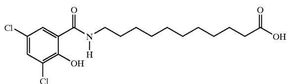
11-N-(3,5-dichloro-2-hydroxybenzoyl)aminoundecanoic acid
