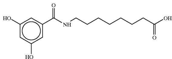
8-(N-(3,5-Dihydroxybenzoyl)aminocaprylic acid
