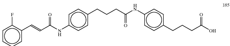
4-(4-(N-(2-Fluorocinnamoyl)aminophenyl)butyric)butyric acid
