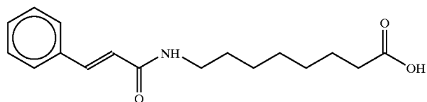
8-cinnamoylaminocaproic acid
