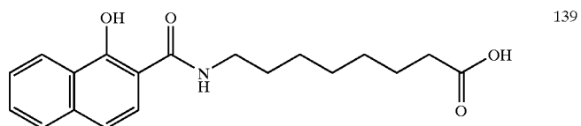
8-(N-(1-hydroxy-2-naphthoyl)aminocaprylic acid
