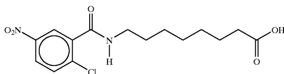
8-(2-chloro-5-nitrobenzoyl)aminocaprylic acid
