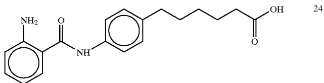
6-(4-(N-2-aminobenzoyl)aminophenyl)hexanoic acid
