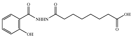
1-salicyloyl-2-suberyl hydrazide
