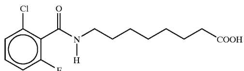
8-N-(2-chloro-6-fluorobenzoyl)]aminocaprylic acid
