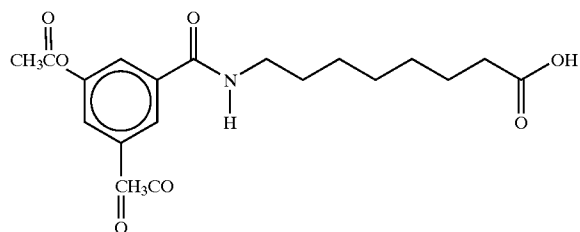
8-(N-(3,5-Diacetyloxybenzoyl)]aminocaprylic acid
