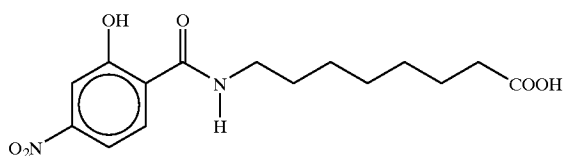
8-(N-(2-hydroxy-4-nitrobenzoyl)aminocaprylic acid
