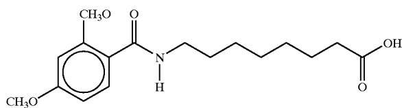
8-(N-2,4-Dihydroxybenzoyl)aminocaprylic acid
