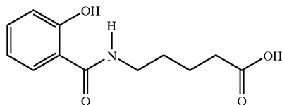
5-(N-salicyloylamino)valeric acid
