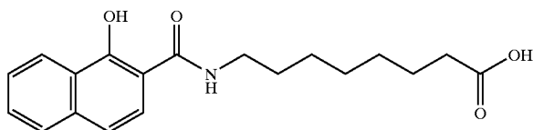
8-(N-1-hydroxy-2-naphthoyl)aminocaprylic acid
