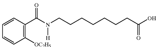
8-(2-ethoxybenzoyl)aminocaprylic acid
