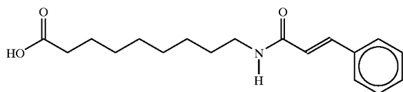
9-(cinnamoylamino)nonanoic acid
