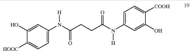
Succinyl-4-aminosalicylic acid
