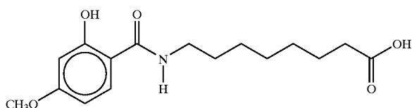
8-(N-2-Hydroxy-4-methoxybenzoyl)aminocaprylic acid
