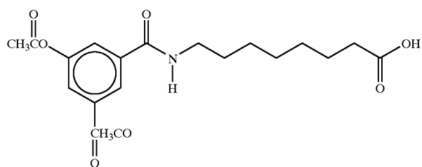
8-(N-3,5-Diacetyloxybenzoyl)aminocaprylic acid
