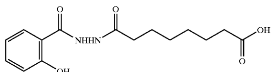
1-salicyloyl-2-suberyl hydrazide
