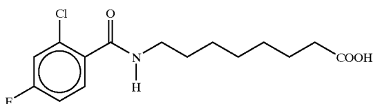
8-(N-2-chloro-4-fluorobenzoyl)aminocaprylic acid
