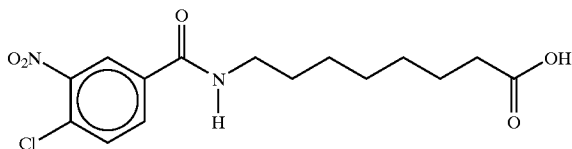
8-(4-chloro-3-nitrobenzoyl)aminocaprylic acid
