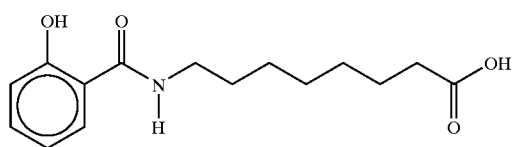
8-(N-(5-methylsalicyloyl)aminocaprylic acid
