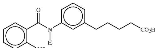
N-Salicyl-5-(3-aminophenyl)valeric acid
