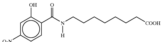
8-(N-(2-hydroxy-4-nitrobenzoyl)aminocaprylic acid
