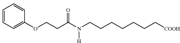
8-(3-Phenoxypropionylamino)caprylic acid
