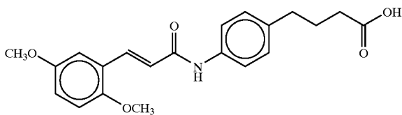
4-(4-(2,5-dimethoxycinnamoyl)aminophenyl)butyric acid
