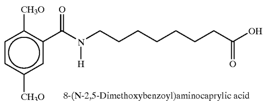
8-(N-2,5-Dimethoxybenzoyl)aminocaprylic acid
