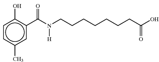
8-(N-(5-methylsalicyloyl)aminocaprylic acid
