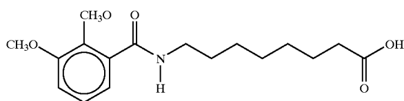
8-(N-2,3-Dimethoxybenzoyl)aminocaprylic acid
