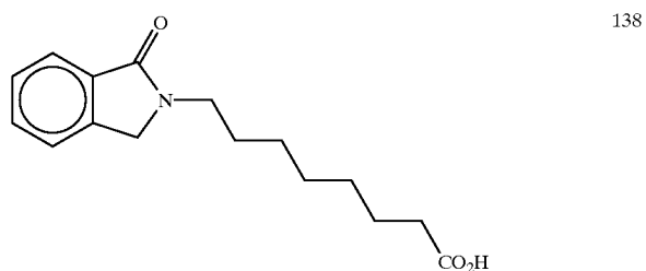
8-(2-(1,2-dihydroisoindole-1-one))octanoic acid
