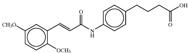
4-(4-(2,5-dimethoxycinnamoyl)aminophenyl)butyric acid
