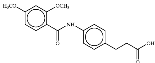
3-[4-(2,4-dimethoxybenzoyl)aminophenyl]propionic acid
