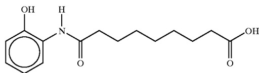
9-(2-hydroxybenzamido)nonanoic acid
