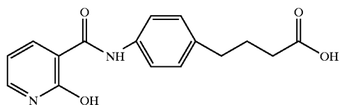
4-(4-(2-hydroxynicotinoyl)aminophenyl)butyric acid
