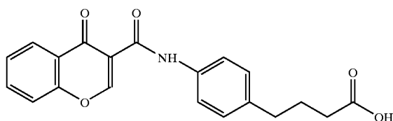
4-(4-(chromone-3-carbonyl)aminophenyl)butyric acid
