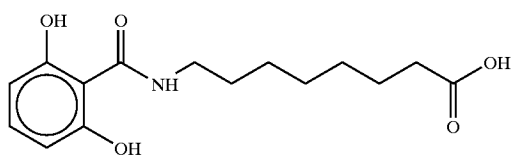
8-(N-(2,6-Dihydroxybenzoyl)aminocaprylic acid
