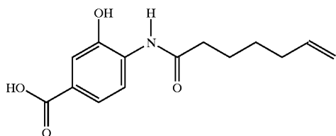
N-(2-hydroxy-4-carboxy)-6-heptenamide
