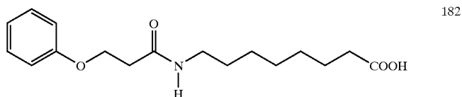
8-(3-Phenoxypropionylamino)caprylic acid
