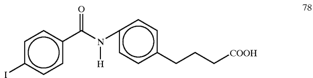
4-{4-[N-(4-iodobenzoyl)]aminophenyl}butyric acid
