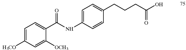
4-(4-(2,4-dimethoxybenzoyl)aminophenyl)butyric acid
