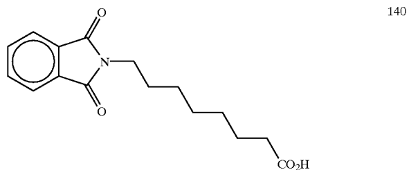
8-(phthalimido)caprylic acid
