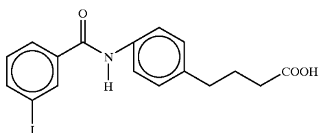
4-[N-[4-(3-iodobenzoyl)aminophenyl]]butyric acid
