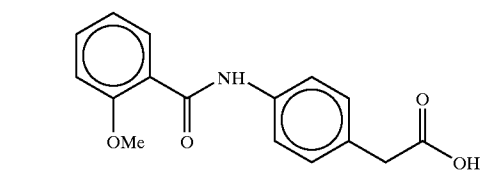
4-(o-anisoyl)aminophenylacetic acid
