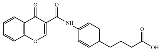
4-(4-(chromone-3-carbonyl)aminophenyl)butyric acid
