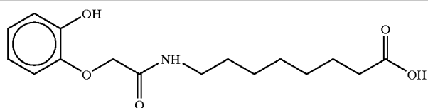
7-(2-hydroxyphenoxyacetyl)aminocaprylic acid
