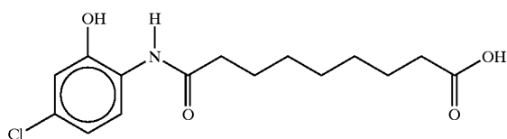
8-(2-hydroxy-5-chloroanilincarbonyl)octanoic acid
