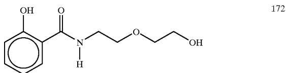
2-[N-(2-hydroxybenzoylamino)ethoxy]ethanol
