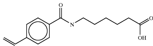
8-(vinylbenzoyl)aminocaproic acid
