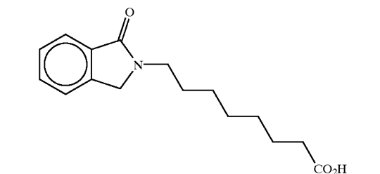
8-(2-(1,2-dihydroisoindole-1-one))octanoic acid
