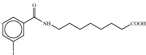
8-N-(3-iodobenzoyl)aminocaprylic acid
