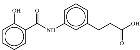
3-(3-(salicyloyl)aminophenyl)propionic acid
