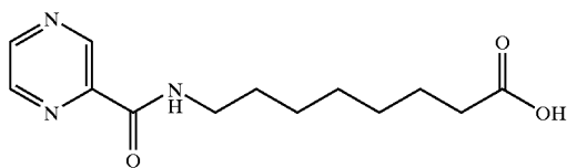
8-(2-pyrazinecarbonyl)aminocaproic acid
