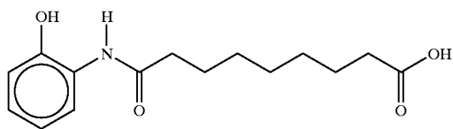
9-(2-hydroxybenzamido)nonanoic acid
