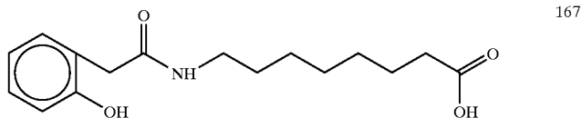
8-(2-hydroxyphenoxy)-aminocaprylic acid
