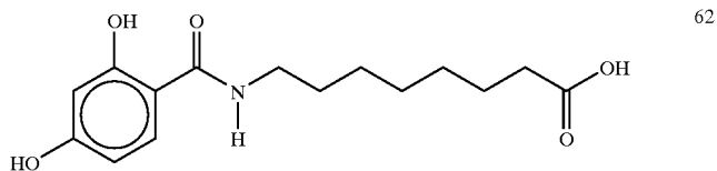
8-(N-2,4-Dihydroxybenzoyl)aminocaprylic acid
