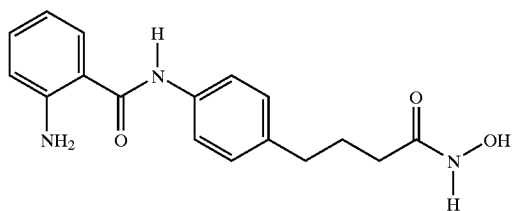
4-[4-(2-aminobenzoylamino)phenyl]butyrylhydroxamic acid
