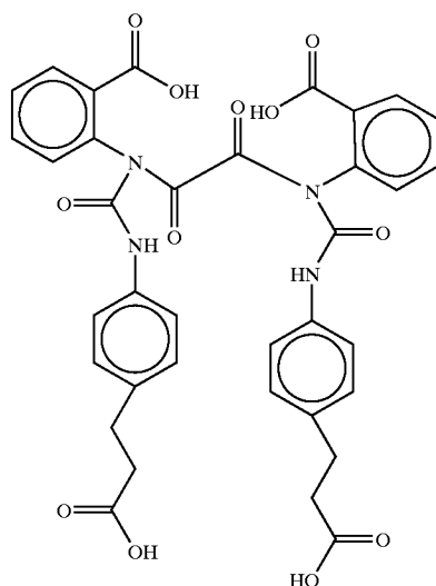
Bis(N-2-carboxyphenyl-N-(N'-3(4-aminophenyl)propionic acid)urea)oxalyldiamide
