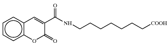
8-[N-(3-coumarincarbonyl)]aminocaproic acid
