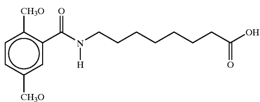
8-(N-(2,5-Dimethoxybenzoyl)]aminocaprylic acid
