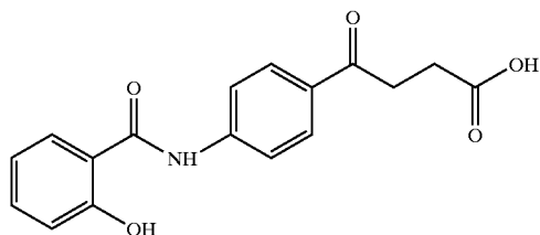
4-(4-salicyloylaminophenyl)-4-oxobutyrlic acid
