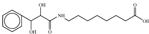
3-phenyl-2,3-dihydroxypropionyl-8-aminocaproic acid
