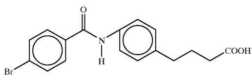
4-[4-[N-(4-bromobenzoyl)aminophenyl]]butyric acid
