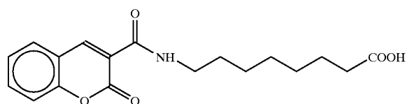
8-[N-(3-coumarincarbonyl)]aminocaproic acid
