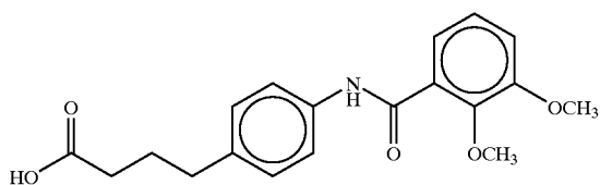
4-(4-(2,3-dimethoxybenzoyl)aminophenyl)butyric acid
