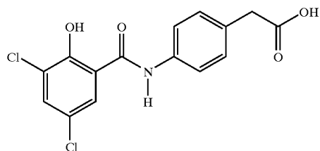
4-[N-(3,5-dichloro-2-hydroxybenzoyl)]aminophenylacetic acid
