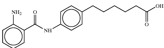
6-(4-(N-2-aminobenzoyl)aminophenyl)hexanoic acid
