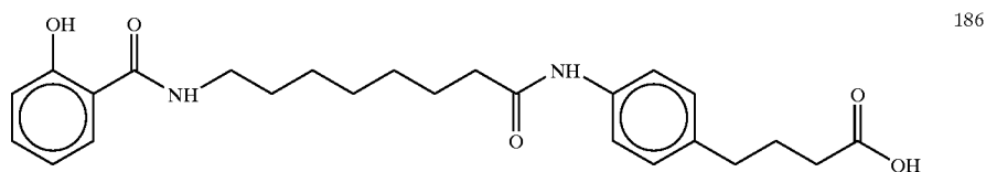
4-(4-(N-(2-Hydroxybenzoyl)-8-aminocaprylic)aminophenyl)butyric acid
