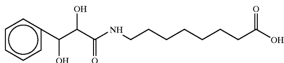
(3-phenyl-2,3-dihydroxypropanoyl)aminocaproic acid
