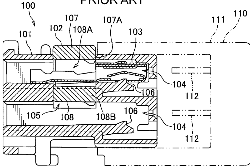
FIG. 7 PRIOR ART
