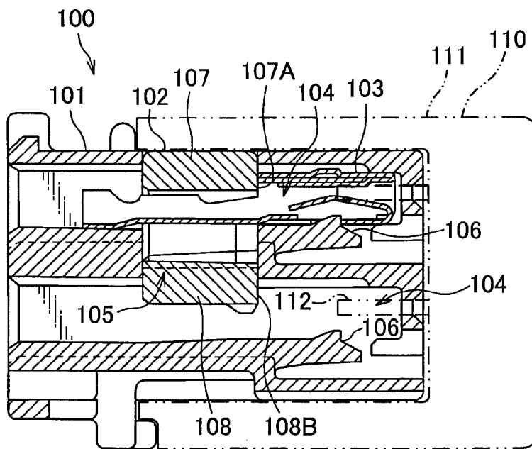
FIG. 9 PRIOR ART
