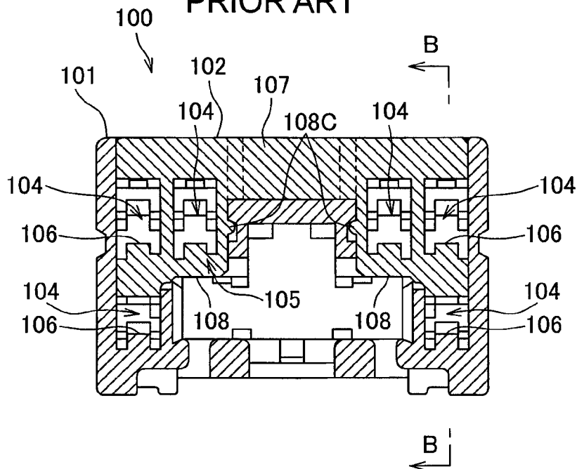
FIG. 8 PRIOR ART
