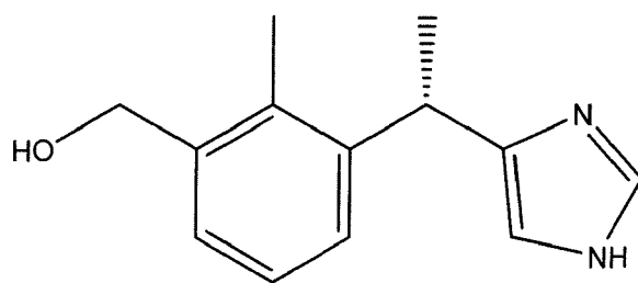
Compound III
