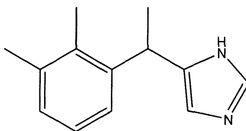
Compound IV
