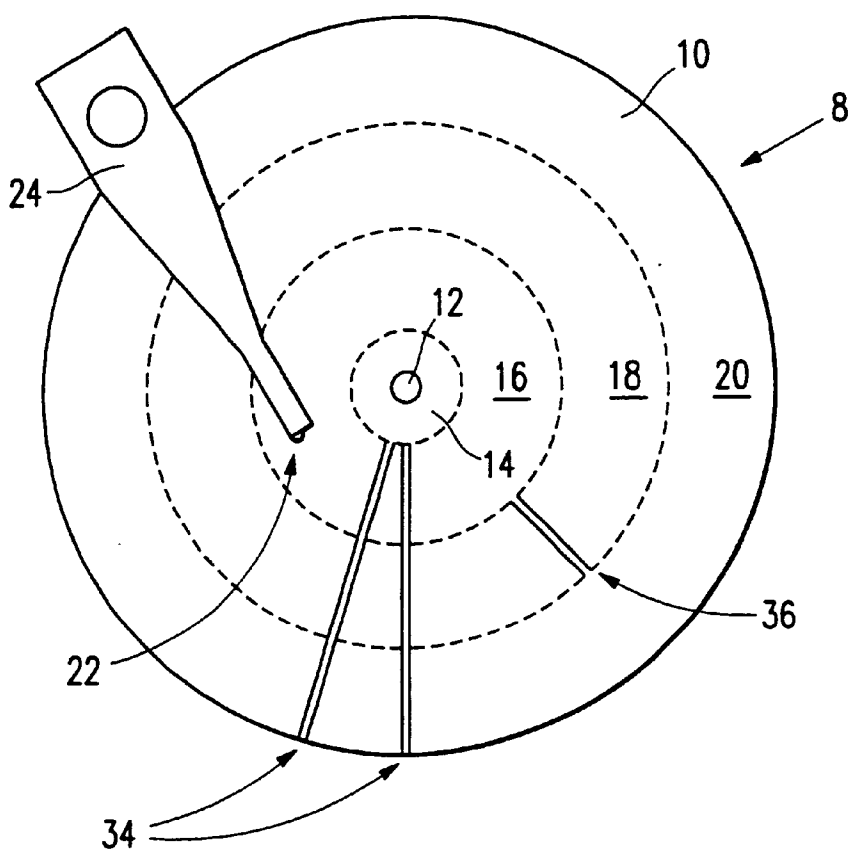
FIG. 7 PRIOR ART
