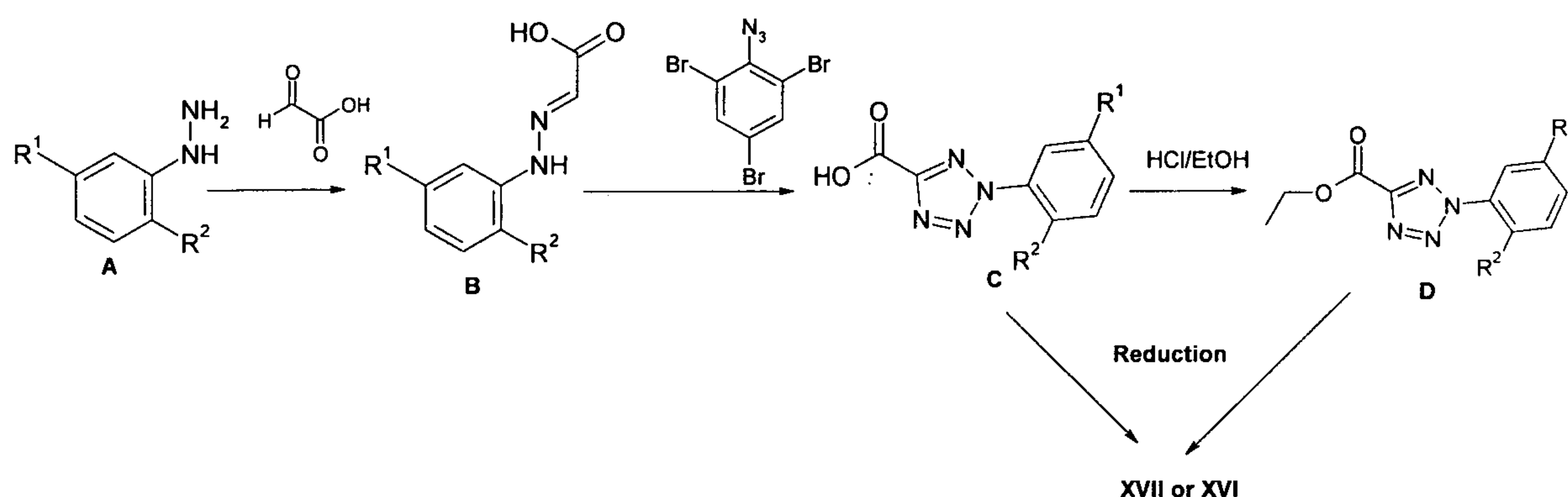
Scheme 5
