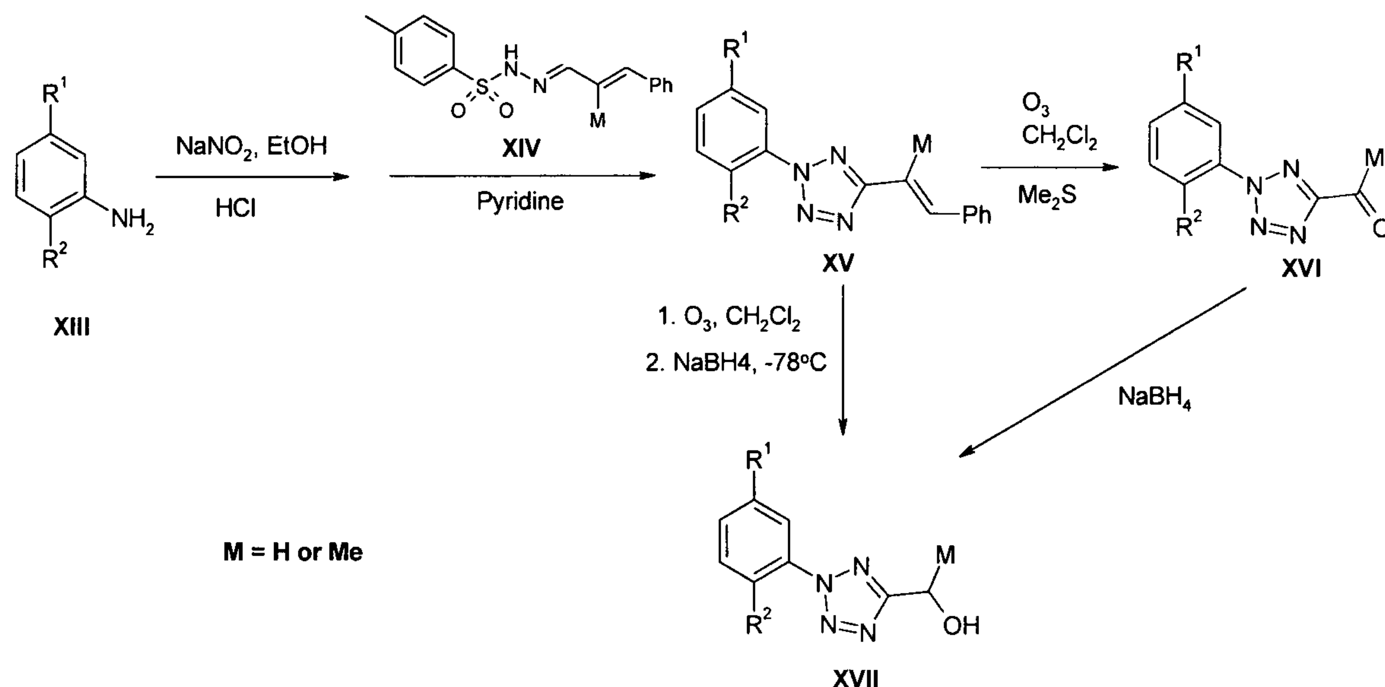
Scheme 4
