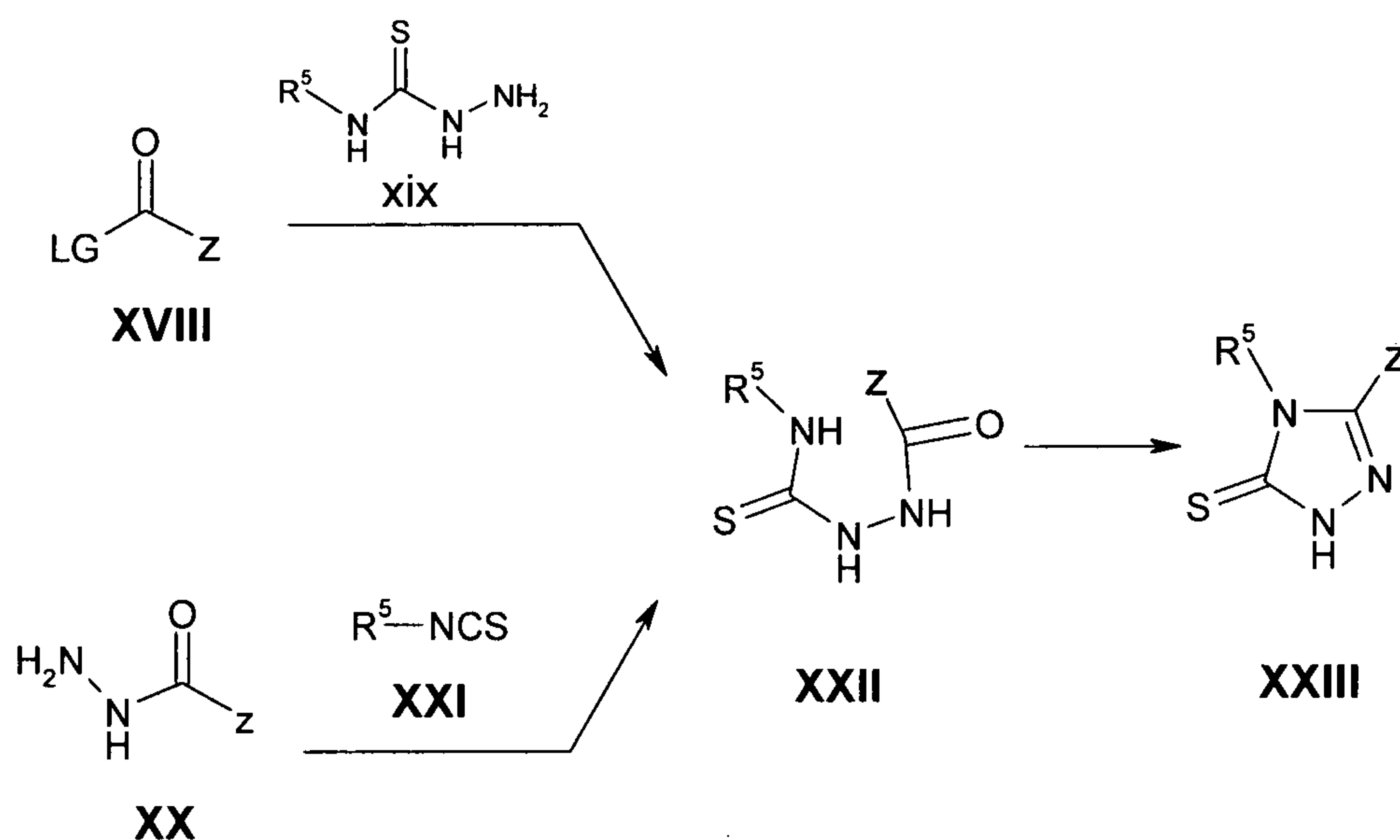
Scheme 6
