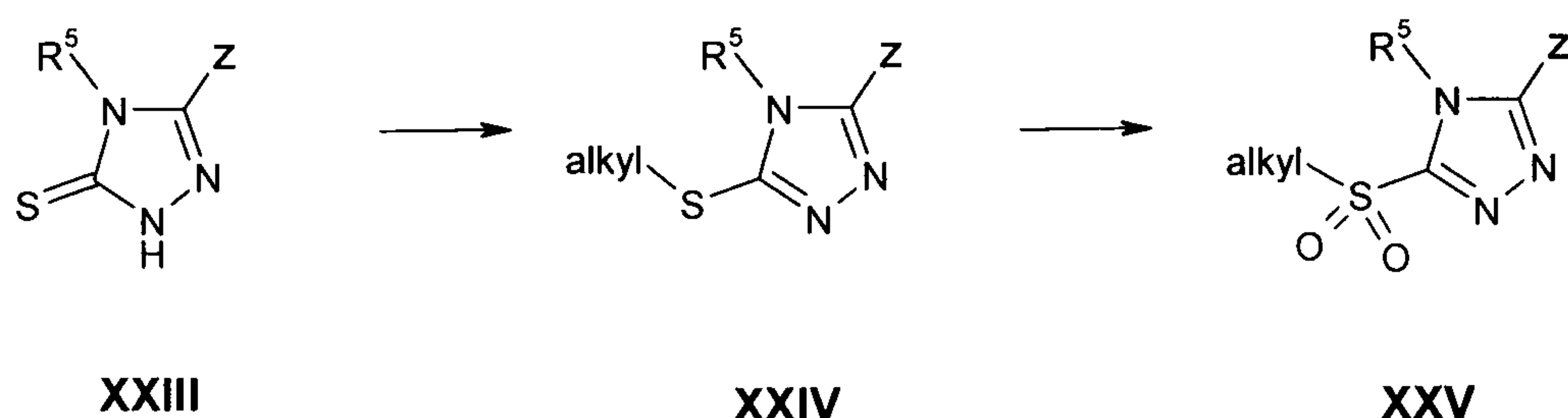
Scheme 7
