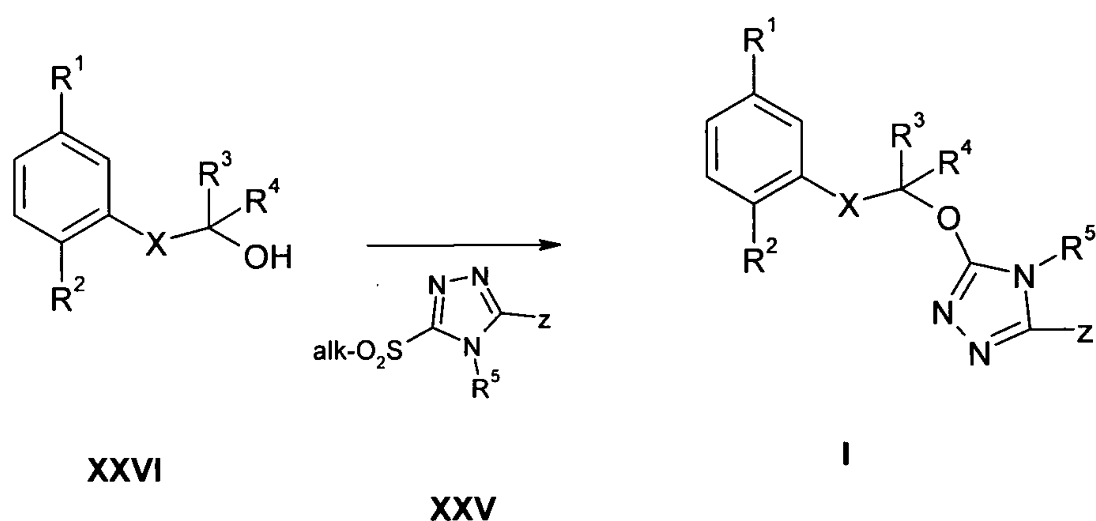
Scheme 8
