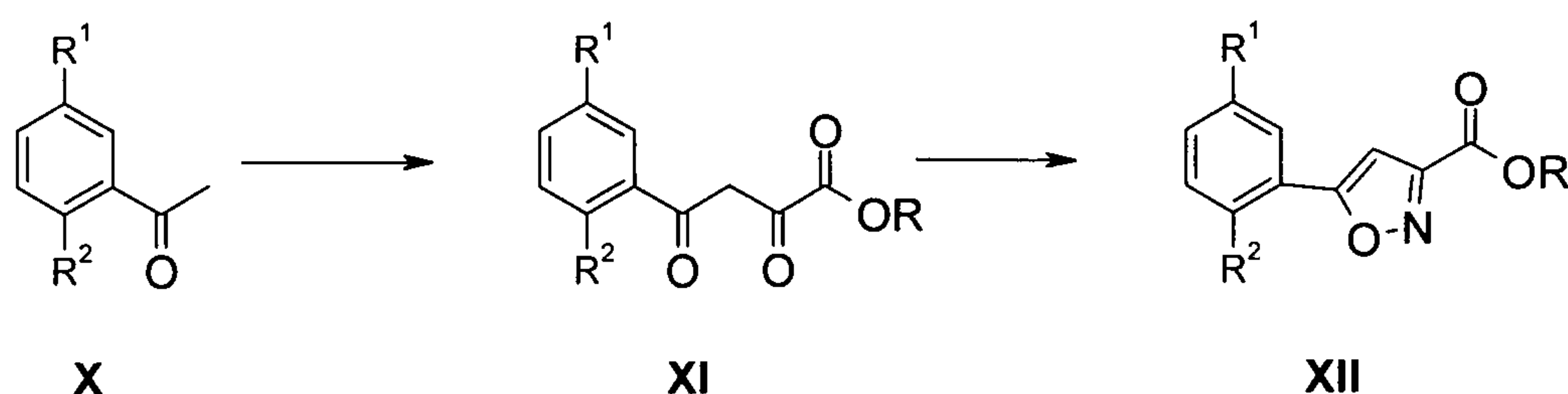
Scheme 3
