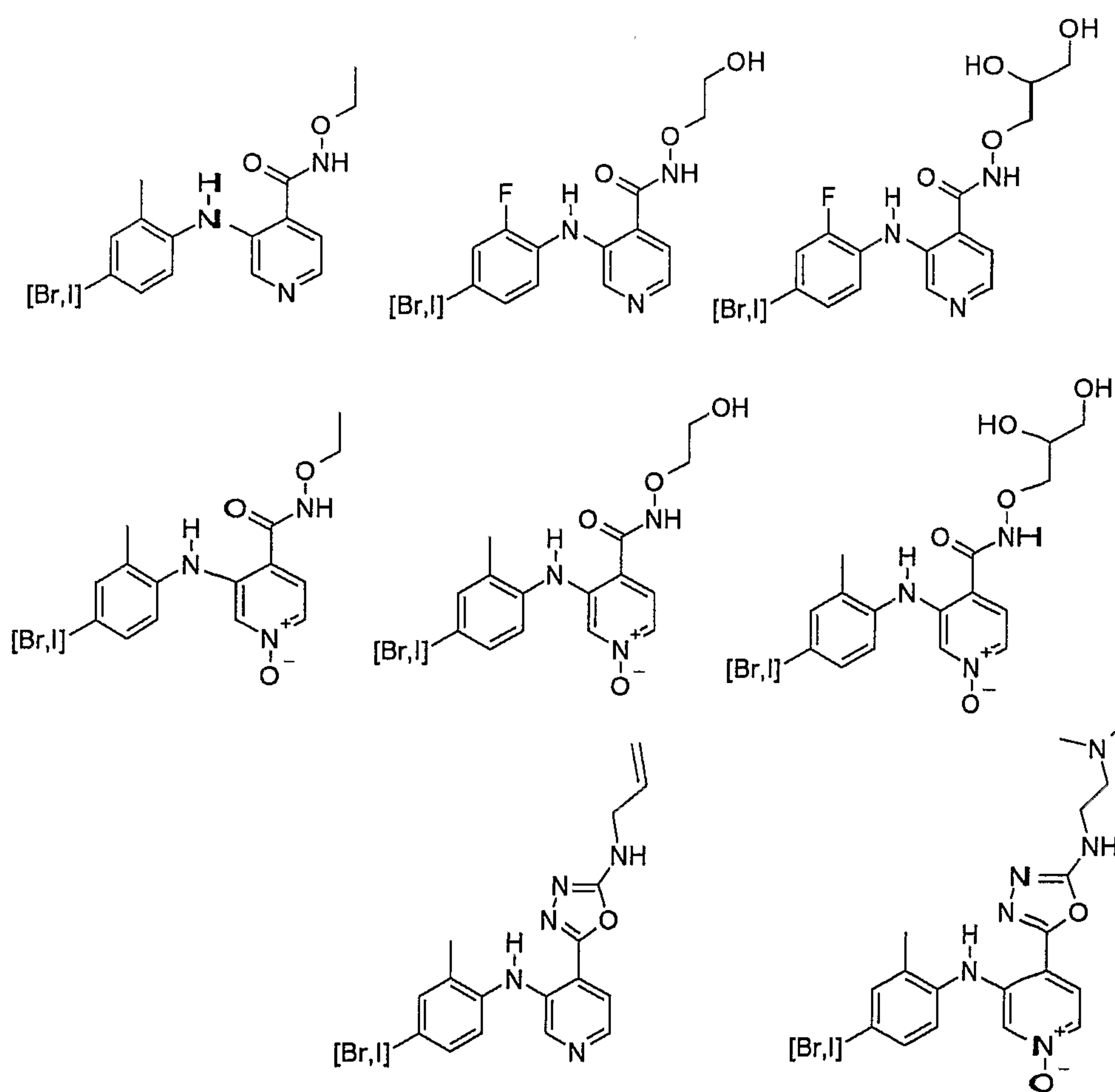
Scheme 1
