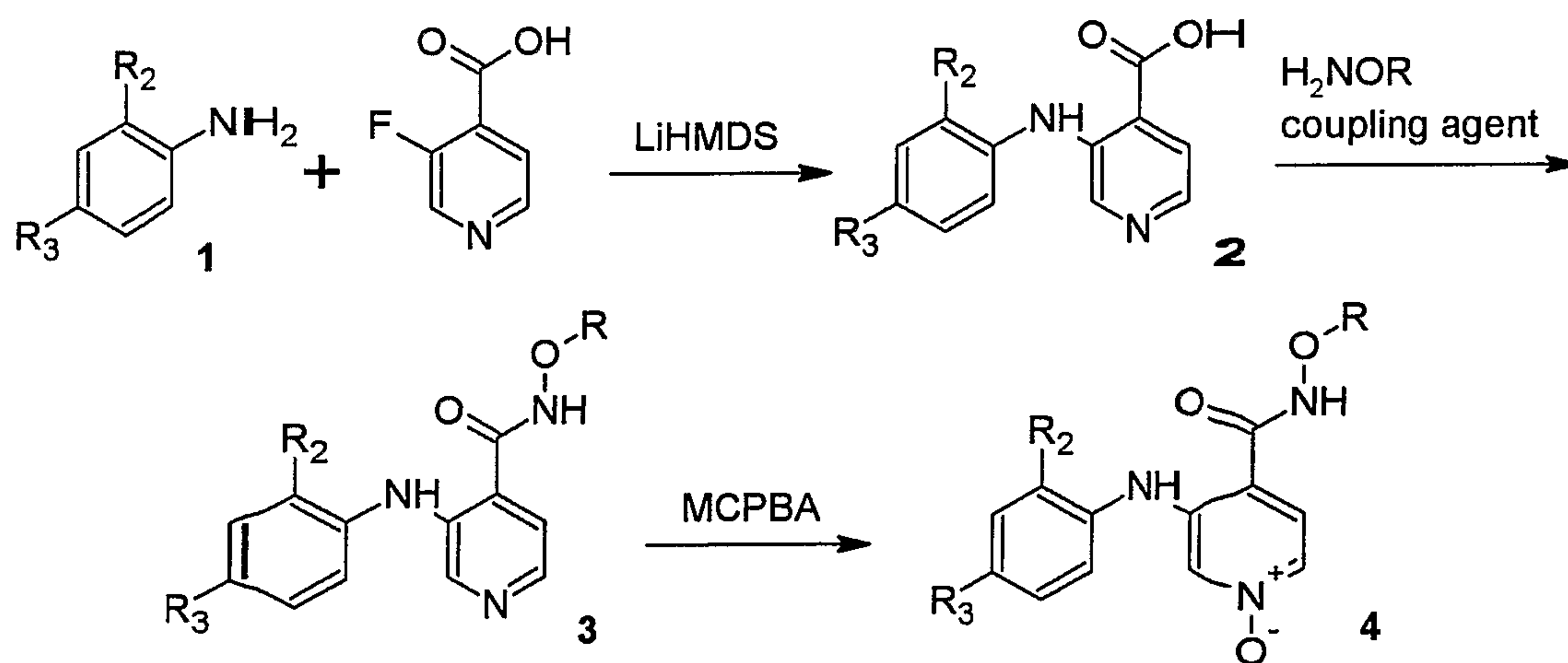
Scheme 2
