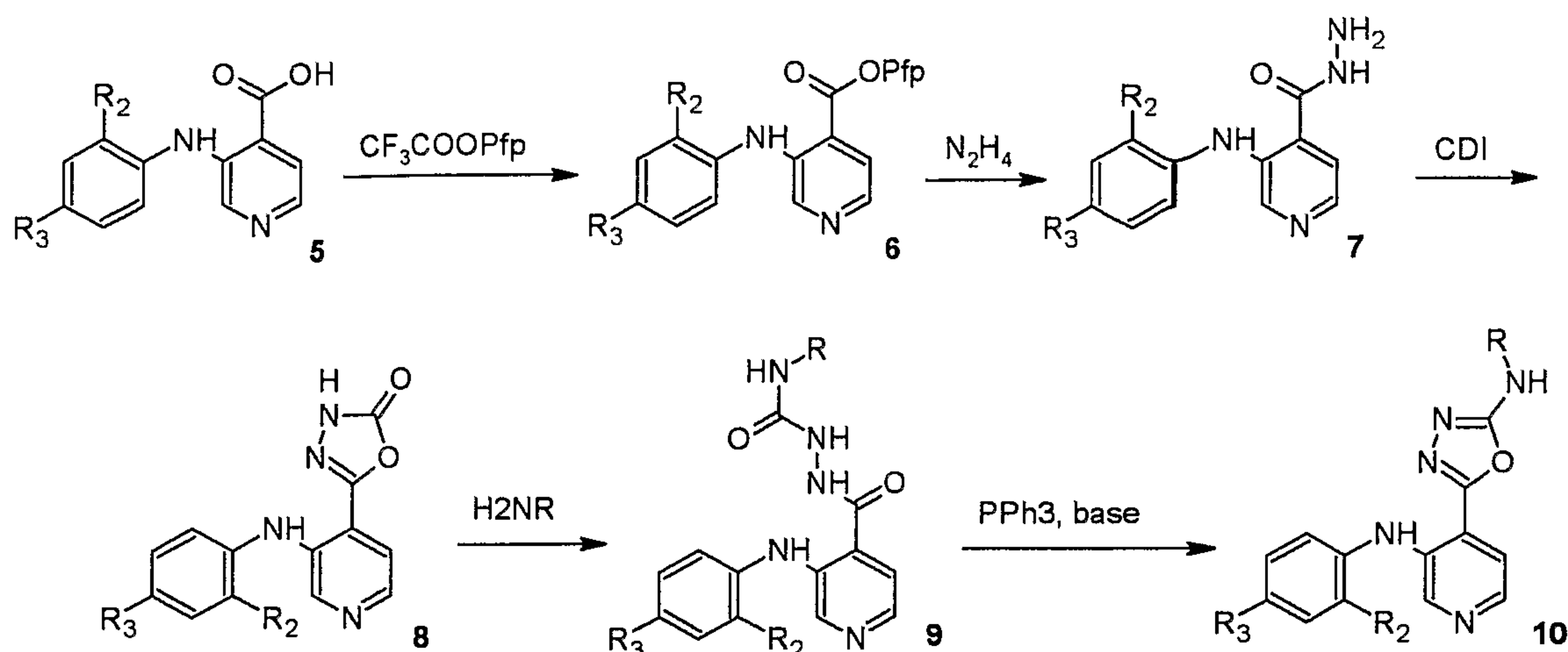
Scheme 3
