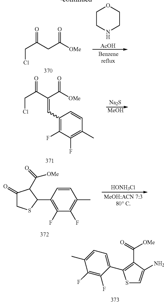
Methyl 4-chloro-2-(2,3-difluoro-4-methylbenzylidene)-3-oxobutanoate (371)
