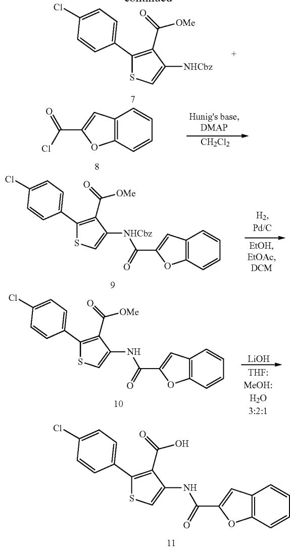
Methyl 4-(((benzyloxy)carbonyl)amino)thiophene-3-carboxylate (3).
