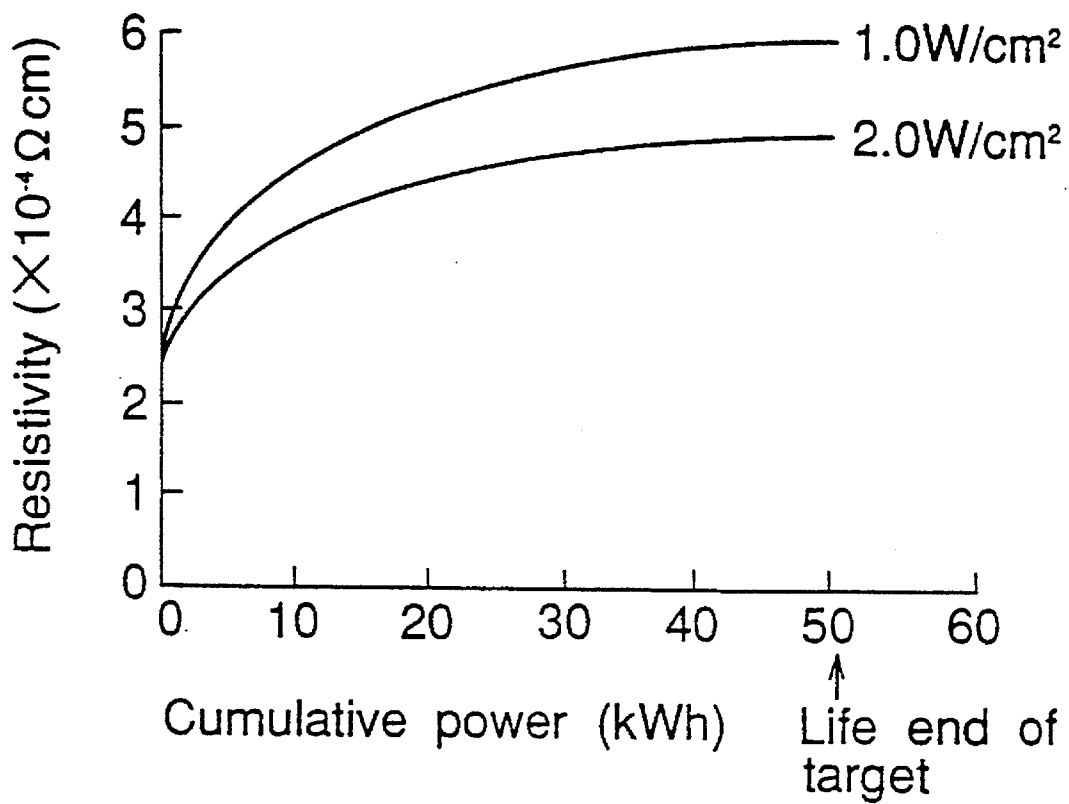
Fig.3 Prior Art
