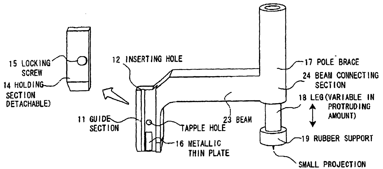
10 DEVICE FOR GUIDING PUNCTURE NEEDLE
