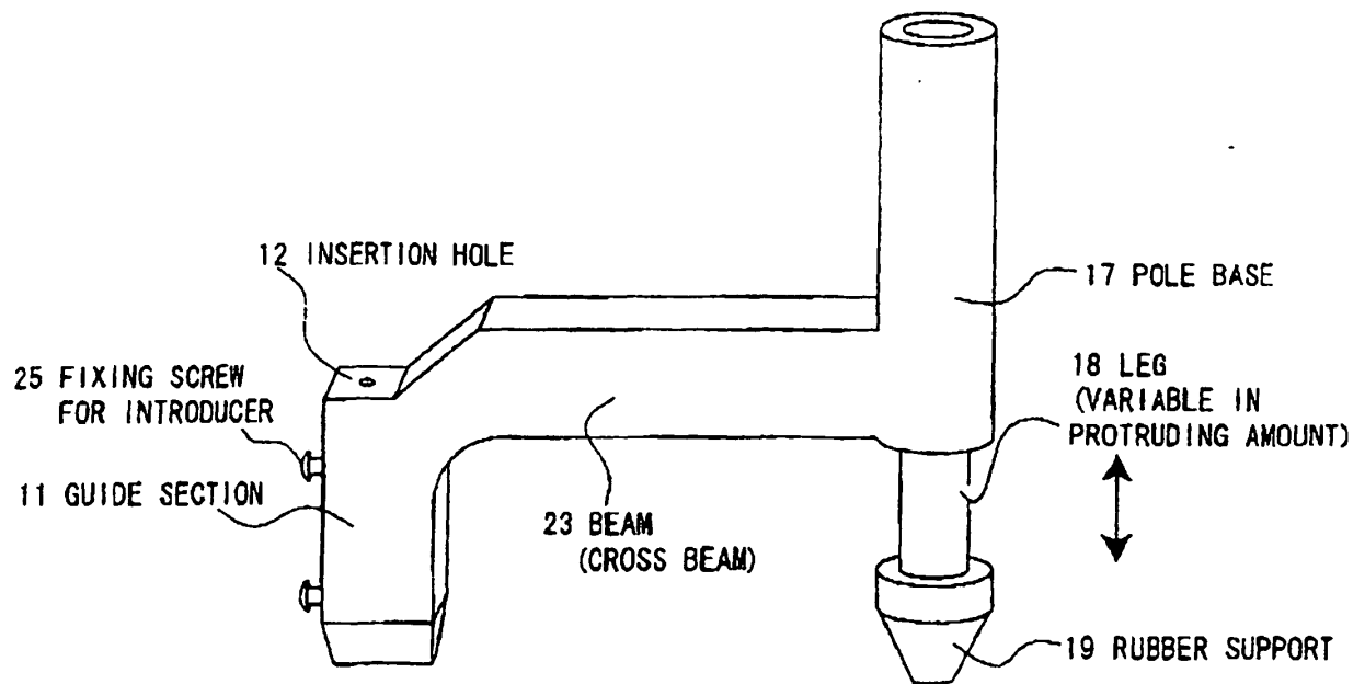
10 DEVICE FOR GUIDING PUNCTURE NEEDLE
