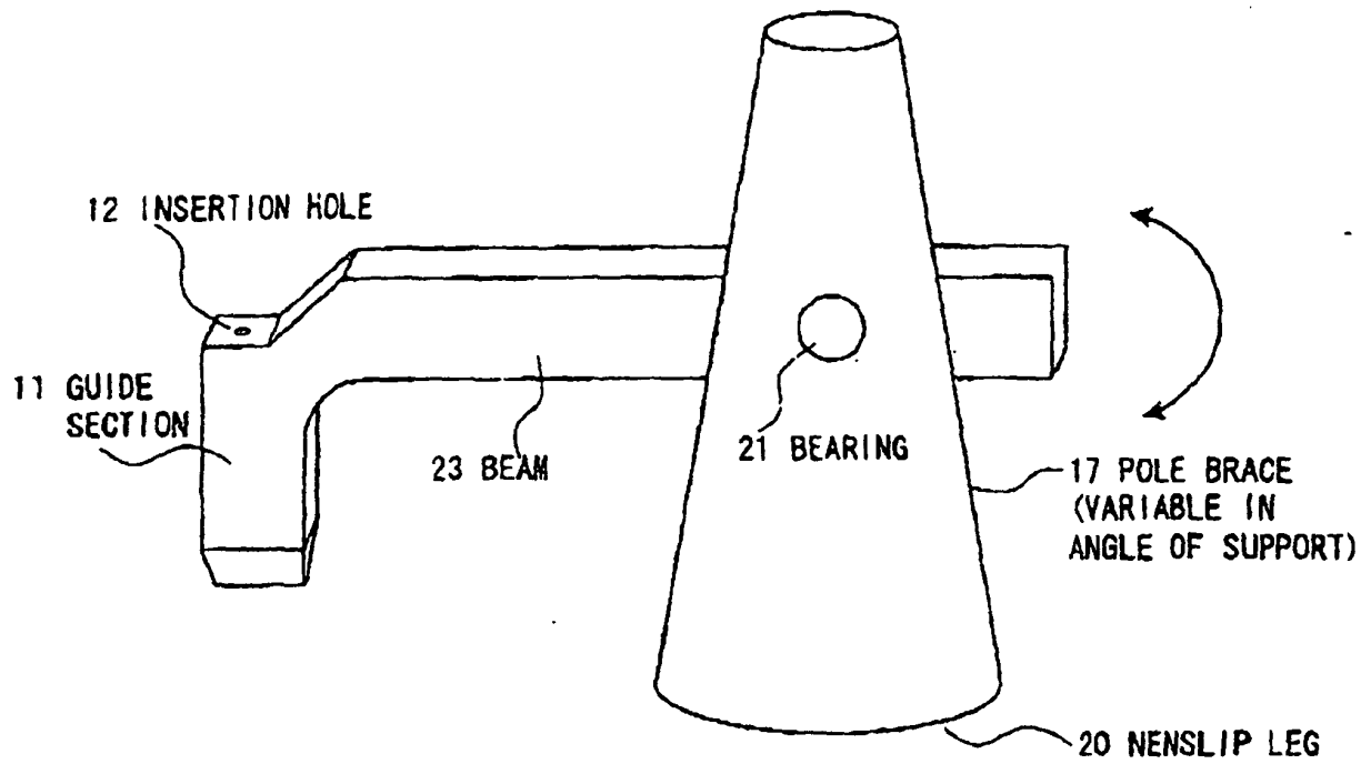
10 DEVICE FOR GUIDING PUNCTURE NEEDLE
