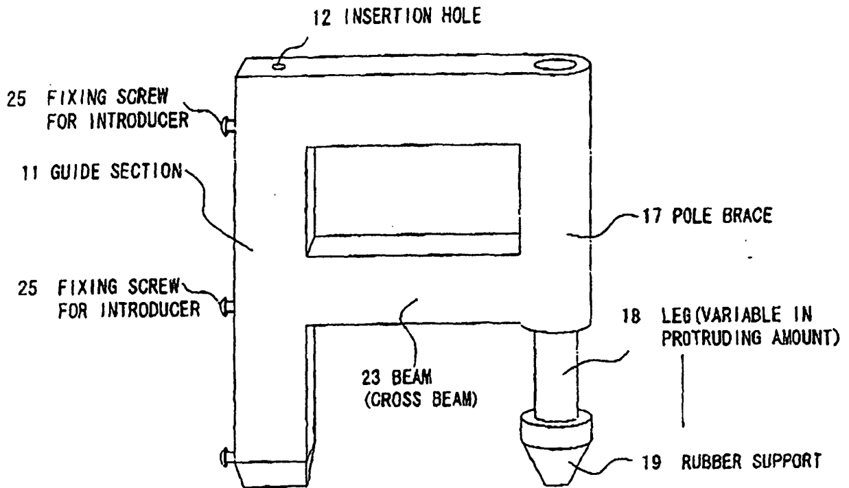
10 DEVICE FOR GUIDING PUNCTURE NEEDLE
