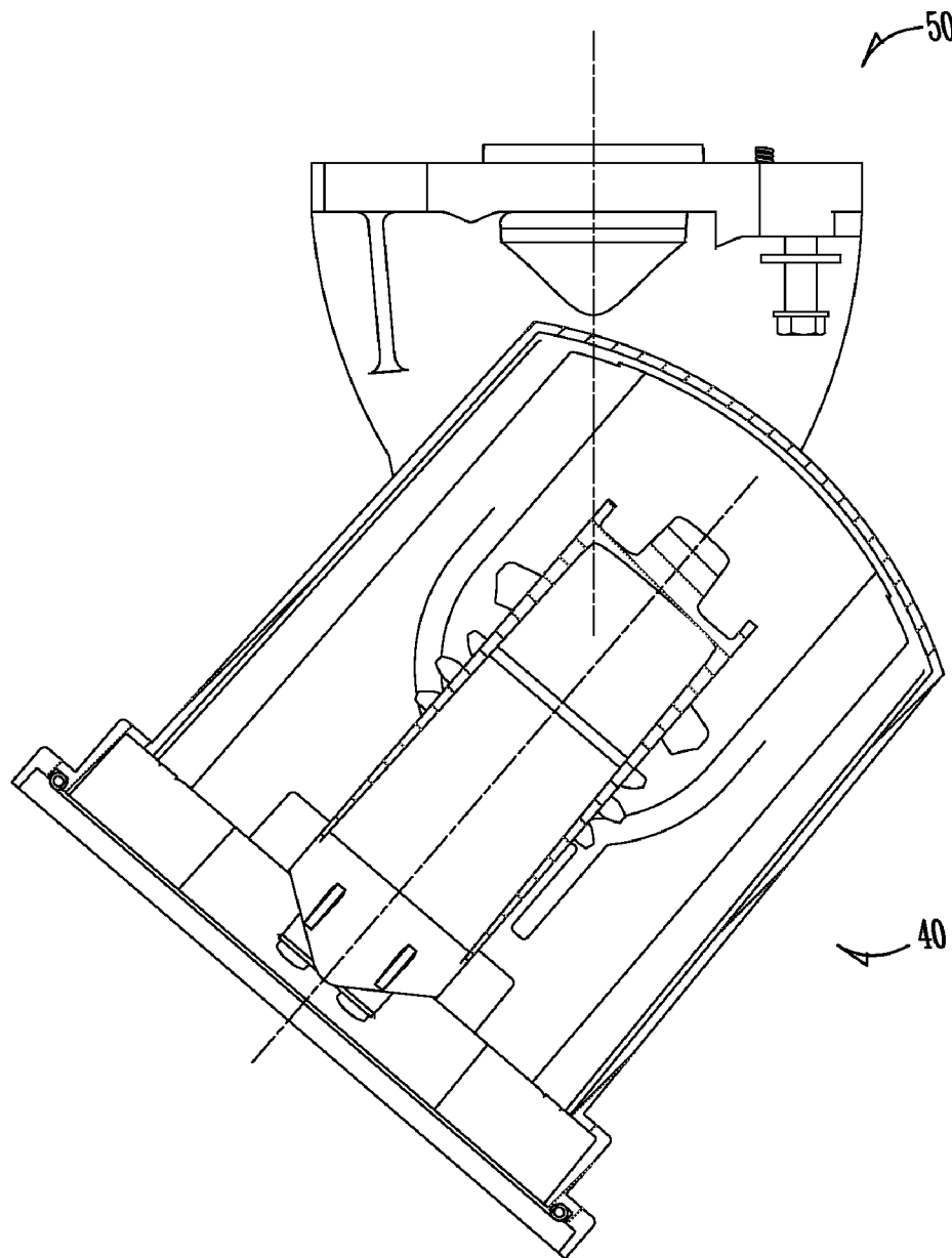
SECTION F-F SHOWN AIMED AT 47° VERTICAL
