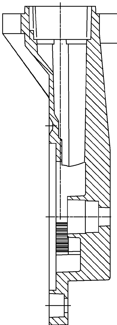
SECTION J-J
