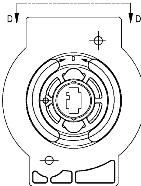
Bottom View Fig. 5D
