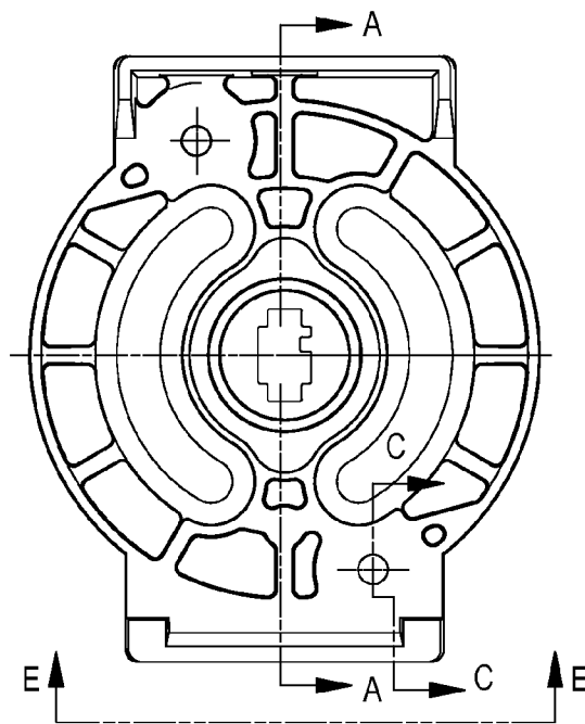
Top View Fig. 5B
