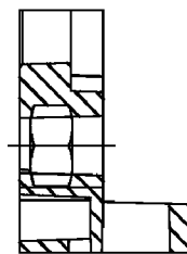
SECTION C-C Fig. 5H
