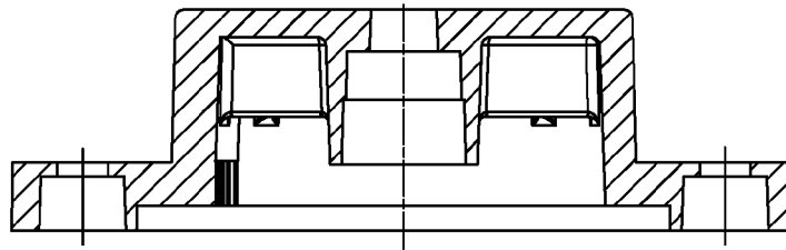
SECTION H-H
