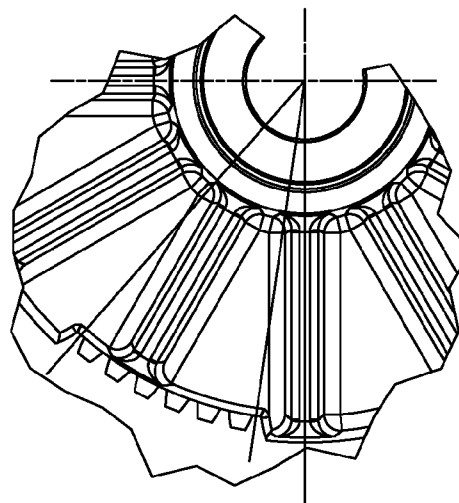
DETAIL K
