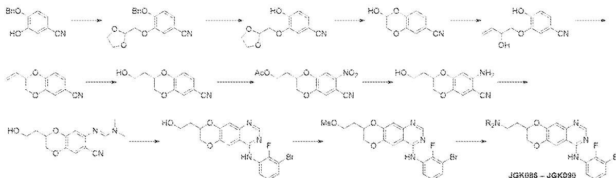
Scheme 8. Synthesis of JGK086-JGK090.
