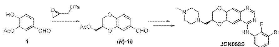
Scheme 3. Synthesis of benzodioxane carbaldehyde ( R )-10 in one step from benzaldehyde 1 with chiral glycidyl tosylate. This route avoids the Mitsunobu reaction in Scheme 1 (preparation of 2 from 1 ). Compound ( R )-10 can be used in the route shown in Scheme 1 for the preparation of JGK068S .
