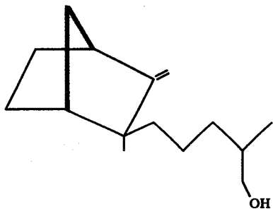
dihydro-beta-santalol
