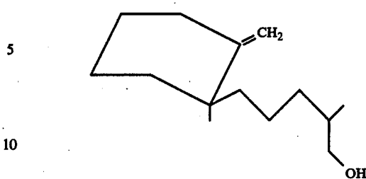
dihydro-beta-santalol
