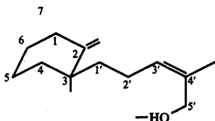
endo-3-methyl-exo-3-(cis-5'-hydroxy-4'-methylpent-3'-enyl)-2-methylenebicyclo[2.2.1]heptane
