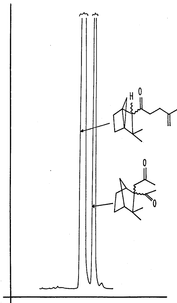
GLC PROFILE FOR EXAMPLE XXXI
