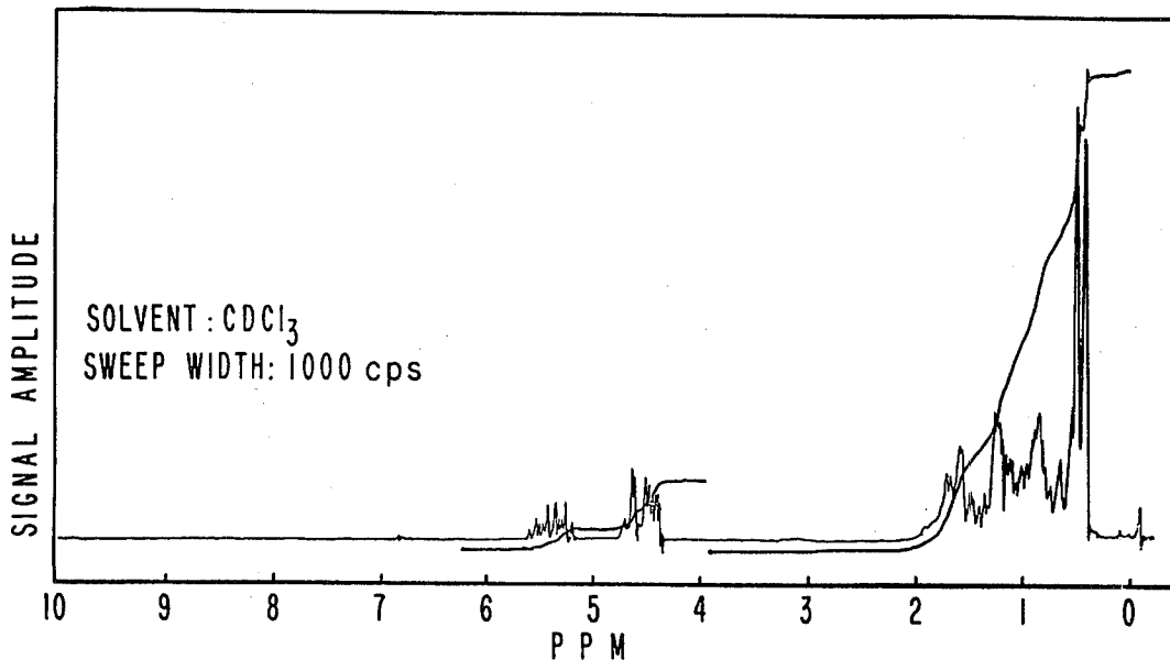
NMR SPECTRUM FOR EXAMPLE II
