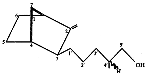
2-methylene-3-exo-(4'-methyl-5'-hydroxypentyl)-bicyclo[2.2.1]heptane; 3-normethyl-dihydro-beta-santalol
