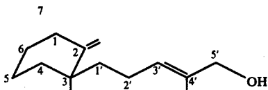
endo-3-methyl-exo-3-(trans-5'-hydroxy-4'-methylpent-3'-enyl)-2-methylenebicyclo[2.2.1]heptane
