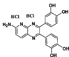
2,3-bis(3,4-dihydroxyphenyl)-pyrido(2,3,b)-pyrazine-6-ylamine, dihydrochloride salt
